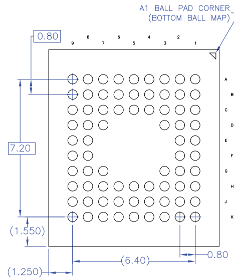
Figure 30. Bottom view
