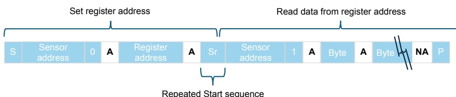
Figure 26. Reliable I 2 C read sequence
