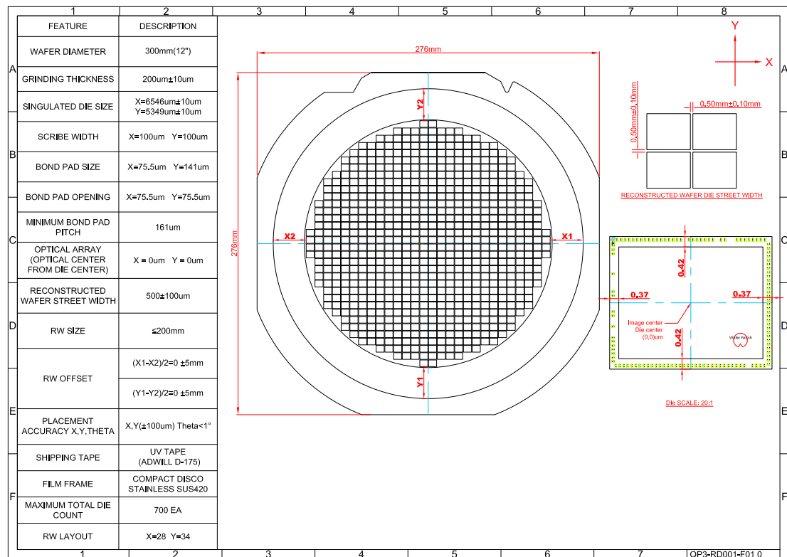
Figure 39. Reconstructed wafer information
