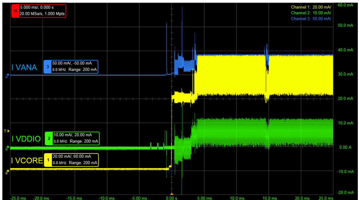
Figure 25. Start streaming and the first frame of typical current profile (mA) over time (ms)
