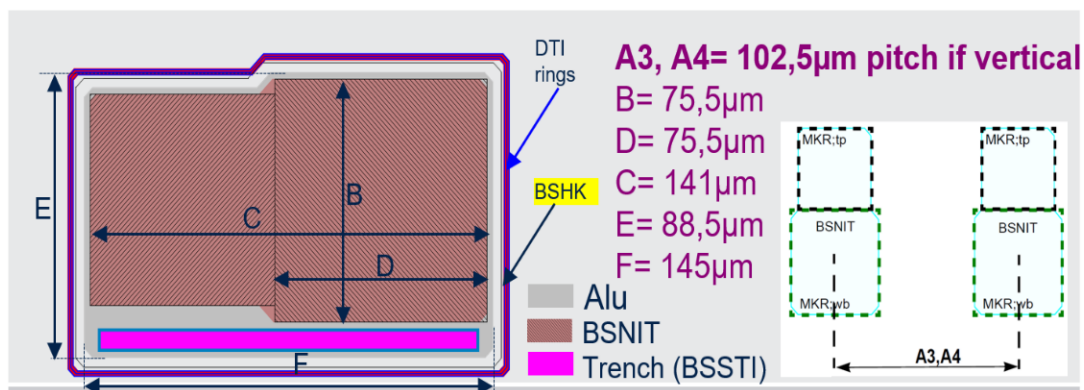
Figure 17. Pad details
