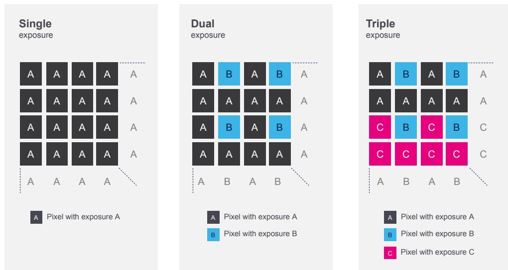
Figure 14. Spatial HDR
