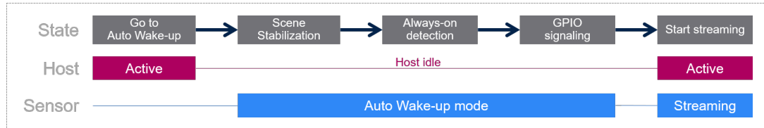
Figure 13. Auto wake-up
