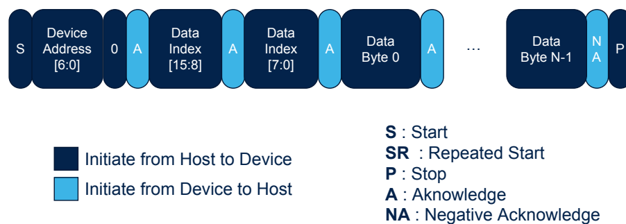
Figure 12. Multibytes write
