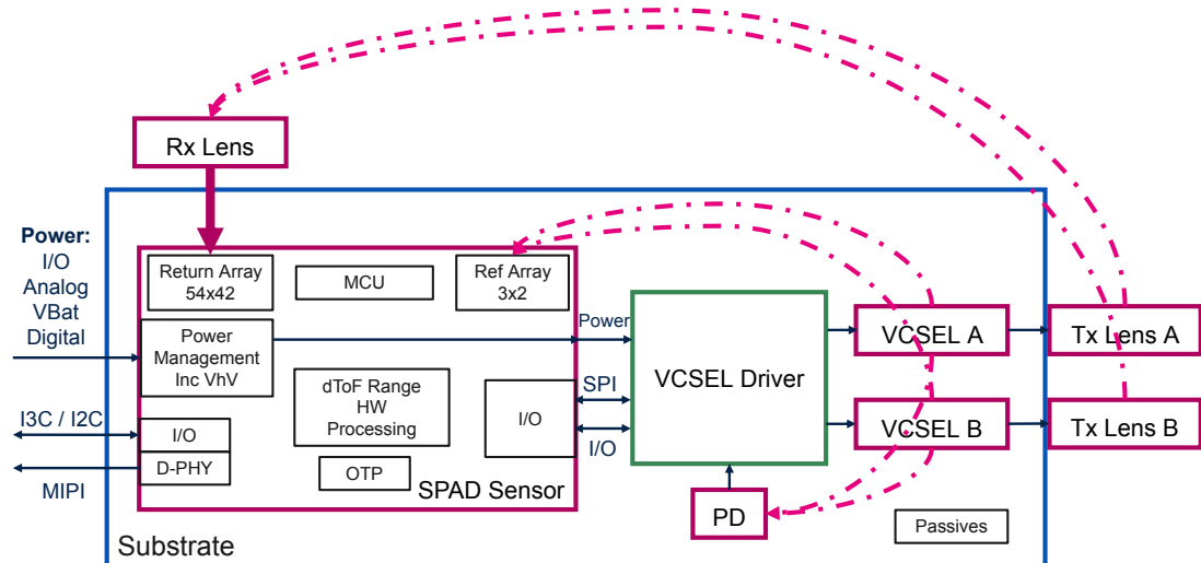
Figure 4. Block diagram
