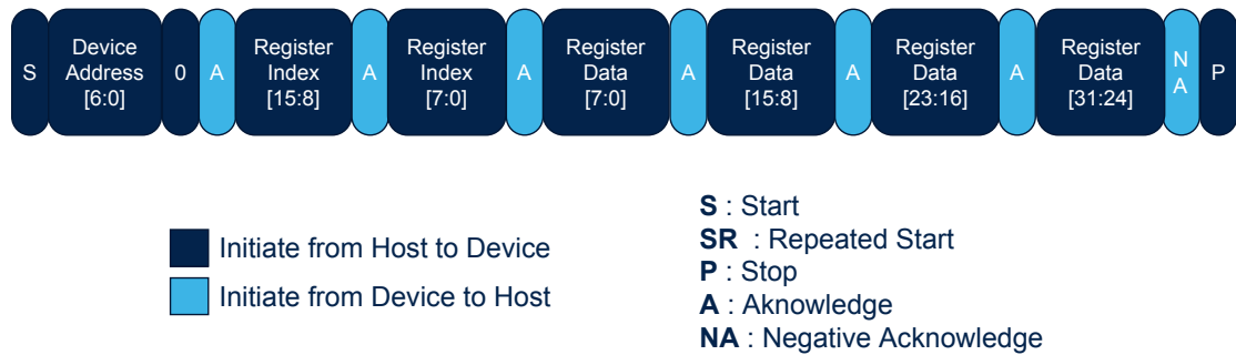
Figure 10. Register write
