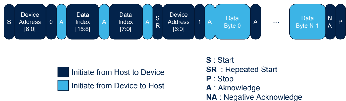
Figure 13. Multibytes read
