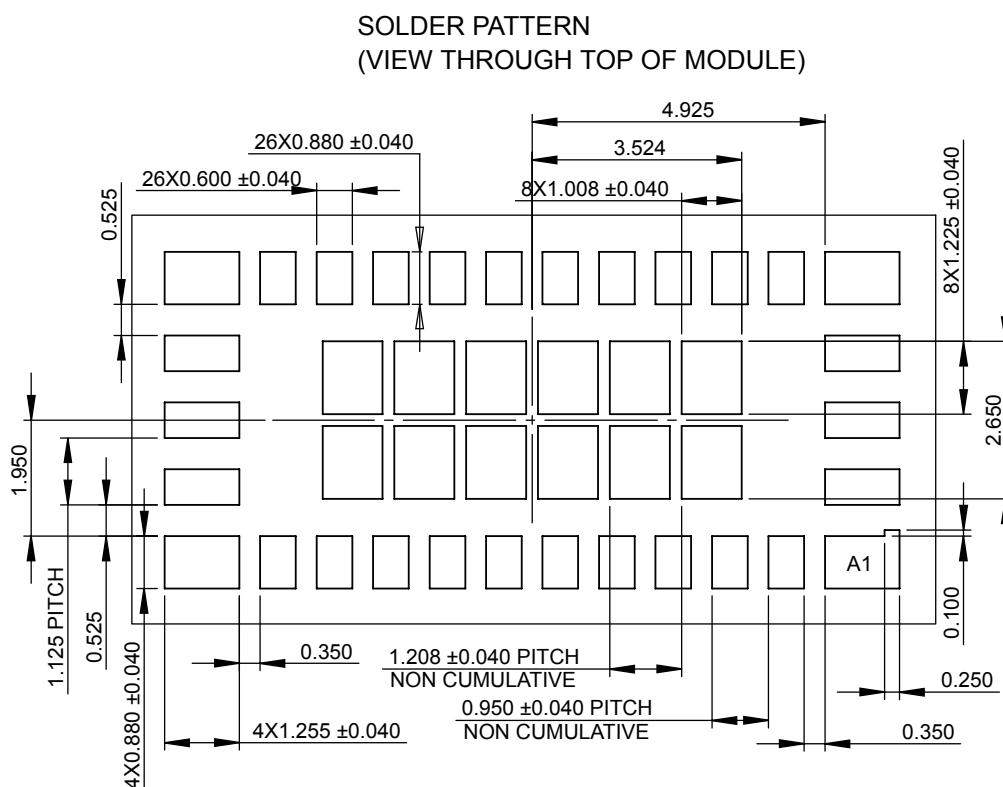
Figure 30. Solder pattern
