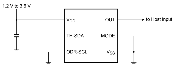
Figure 15. Standalone mode, Low threshold, Medium sample rate
