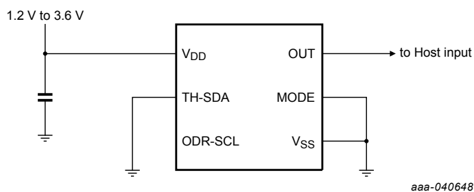
Figure 19. Standalone mode, Medium threshold, Low sample rate
