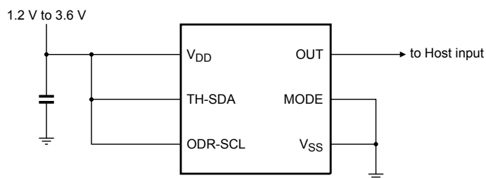
Figure 14. Standalone mode, High threshold, High sample rate
