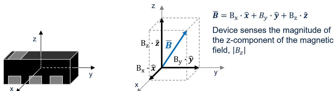
Figure 3. Magnetic field sensitivity vs. package orientation
