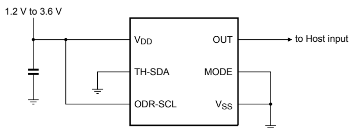
Figure 13. Standalone mode, Medium threshold, High sample rate
