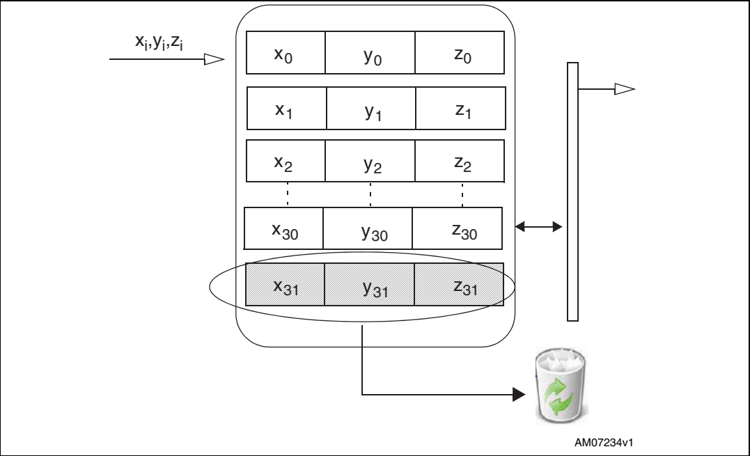
Figure 9. Stream mode
