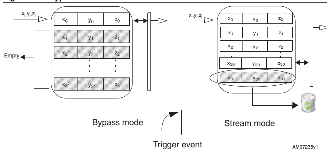
Figure 10. Bypass-to-stream mode
