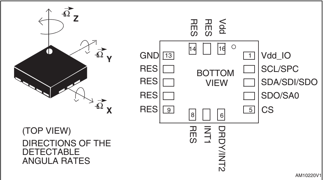
Figure 2. Pin connection
