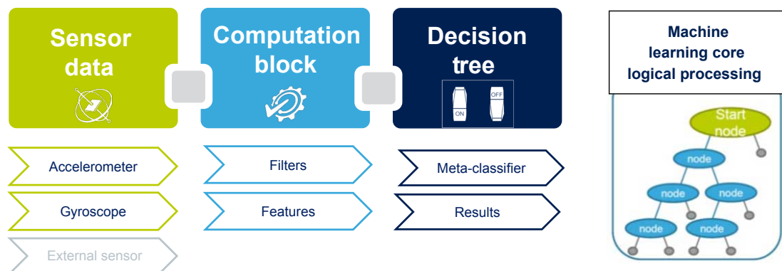
Figure 4. Machine learning core in the LSM6DSV80X
