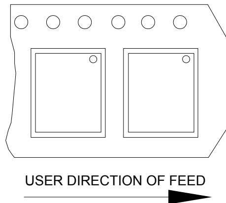
Figure 26. LGA-14L package orientation in carrier tape
