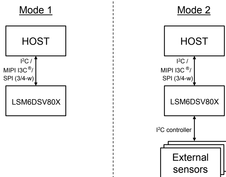
Figure 6. LSM6DSV80X connection modes
