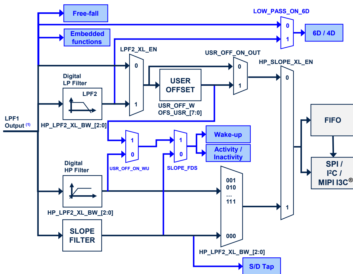
Figure 23. Low-g accelerometer composite filter
