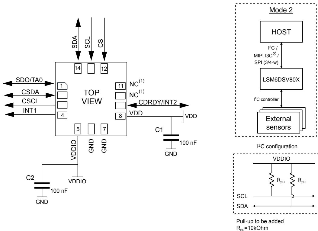
Figure 22. LSM6DSV80X electrical connections in mode 2
