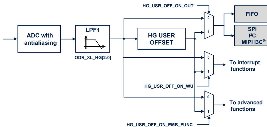
Figure 19. High-g accelerometer filtering chain
