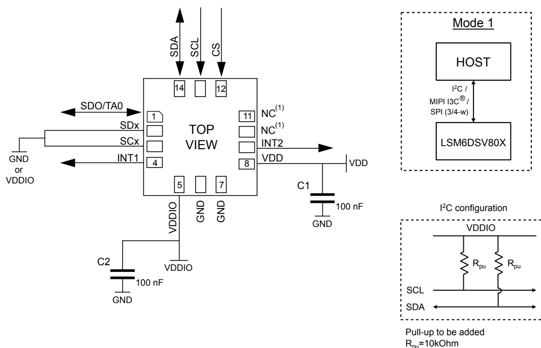
Figure 21. LSM6DSV80X electrical connections in mode 1
