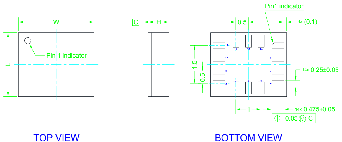
Figure 24. LGA-14L 2.5 x 3.0 x 0.83 mm package outline and mechanical data
