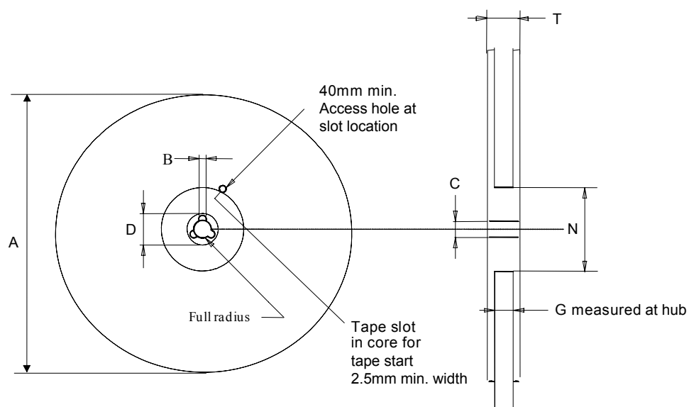
Figure 27. Reel information for carrier tape of LGA-14L package
