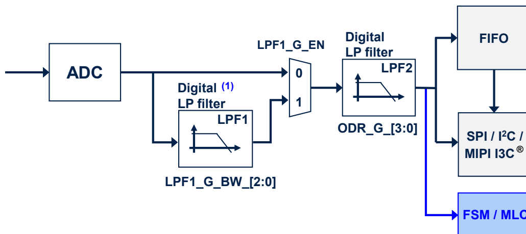
Figure 20. Gyroscope digital chain
