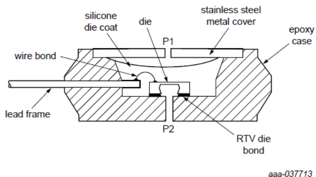
Figure 8. Unibody package — cross-sectional diagram (not to scale)
