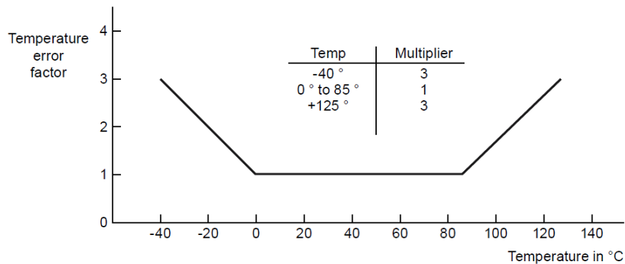
Figure 9. Temperature error band
