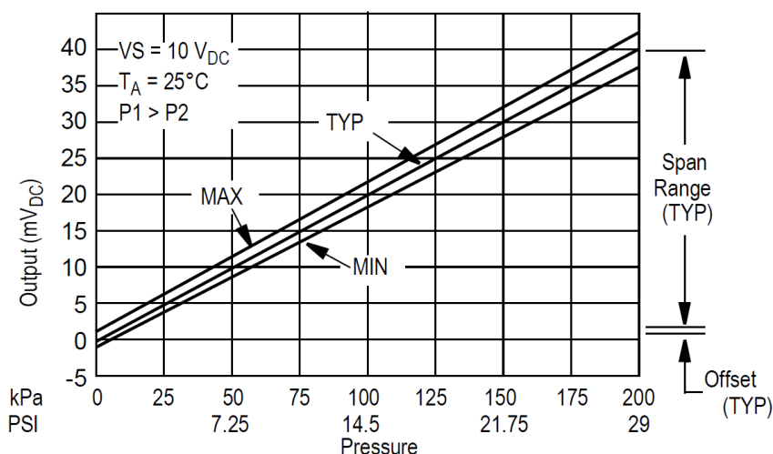
Figure 2. Output vs. Pressure Differential
