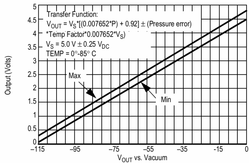
Figure 6. Transfer function
