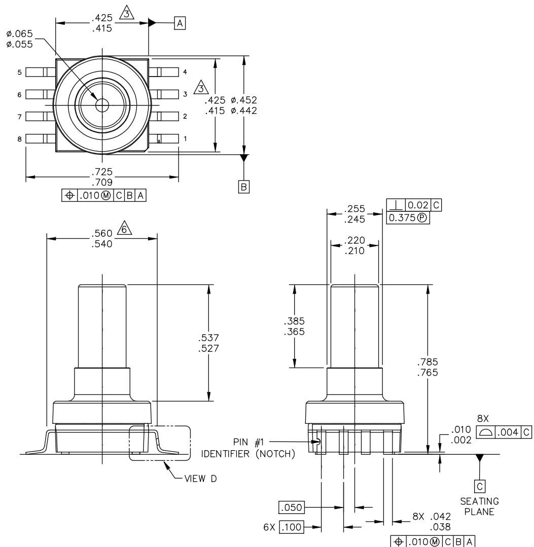
Figure 19. SOT1691-2 Package Outline
