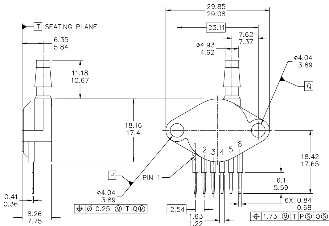
Figure 27. SOT1852-1 Package Outline
