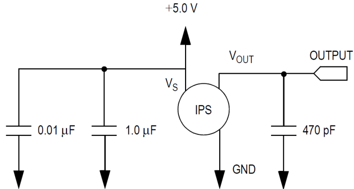
Figure 7. Recommended power supply decoupling and output filtering (For additional output filtering, please refer to application note AN1646.)
