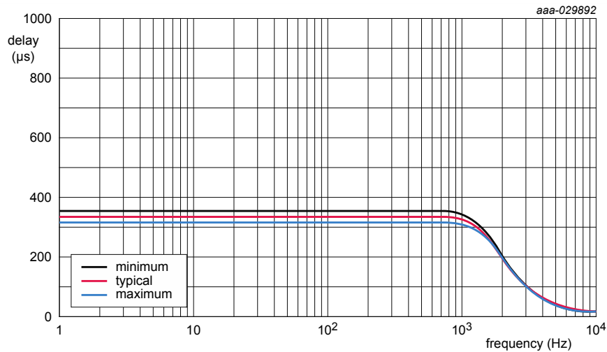
Figure 11. 1000 Hz, 4-pole output signal delay
