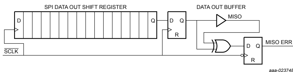
Figure 21. SPI data output verification
