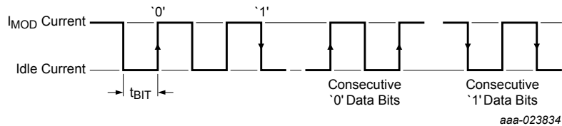
Figure 48. Manchester data bit encoding
