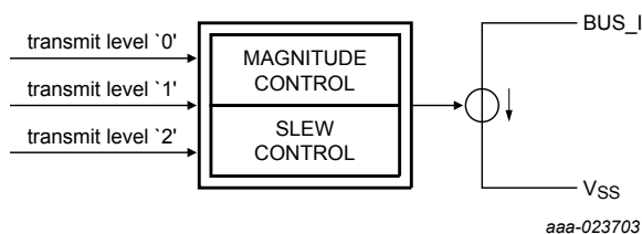
Figure 27. DSI3 transmitter block diagram
