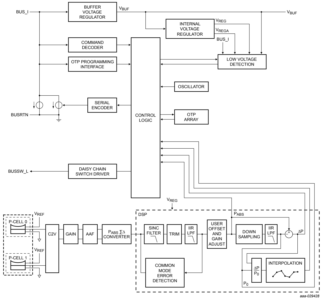
Figure 1. Block diagram
