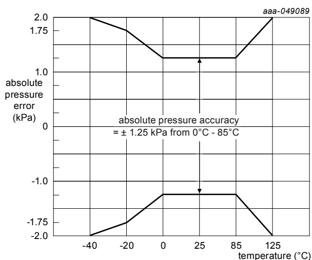
Figure 22. Absolute pressure accuracy as a function of temperature
