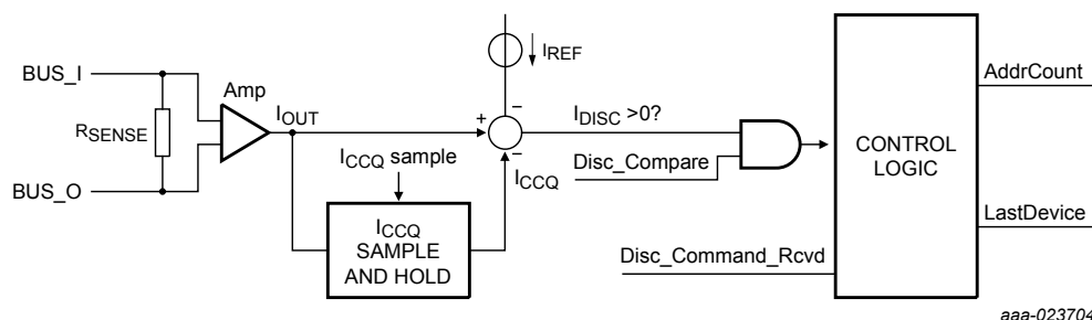
Figure 28. Discovery mode current sense circuit block diagram
