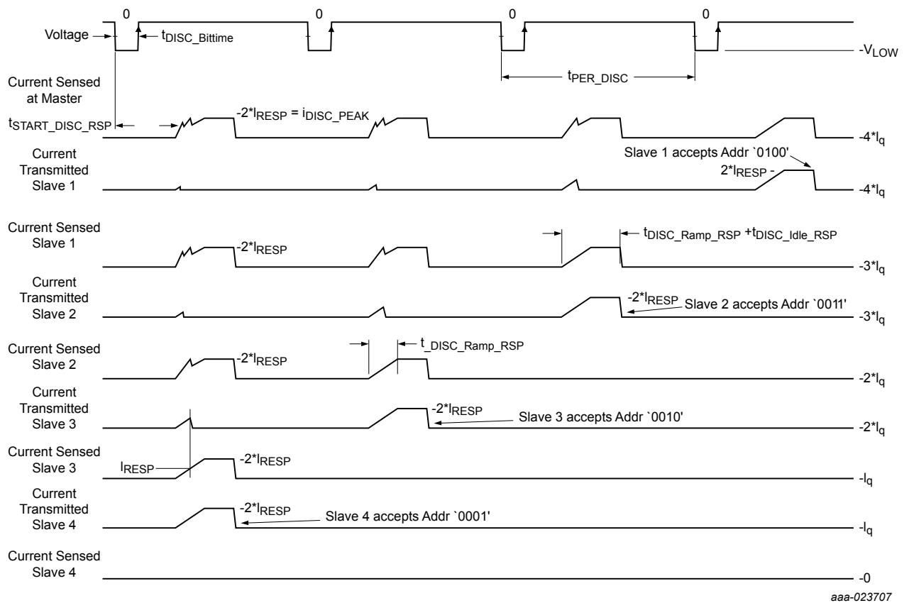
Figure 30. DSI3 discovery mode timing diagram
