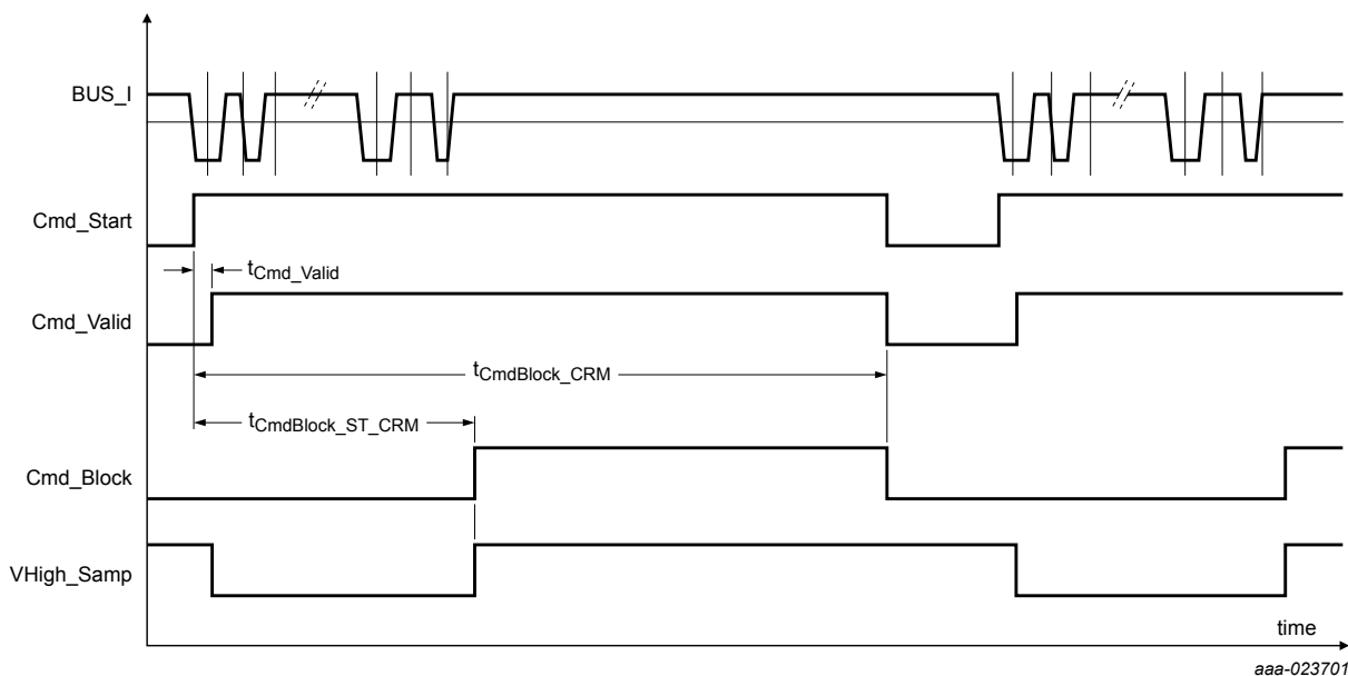
Figure 25. DSI3 command receiver timing diagram: valid command
