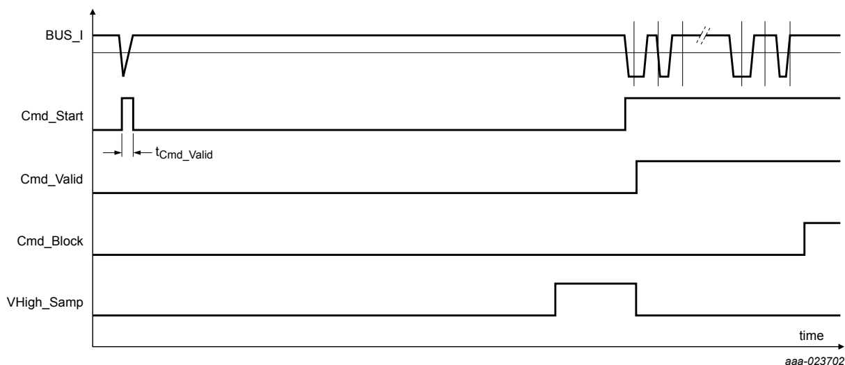
Figure 26. DSI3 command receiver timing diagram: microcut
