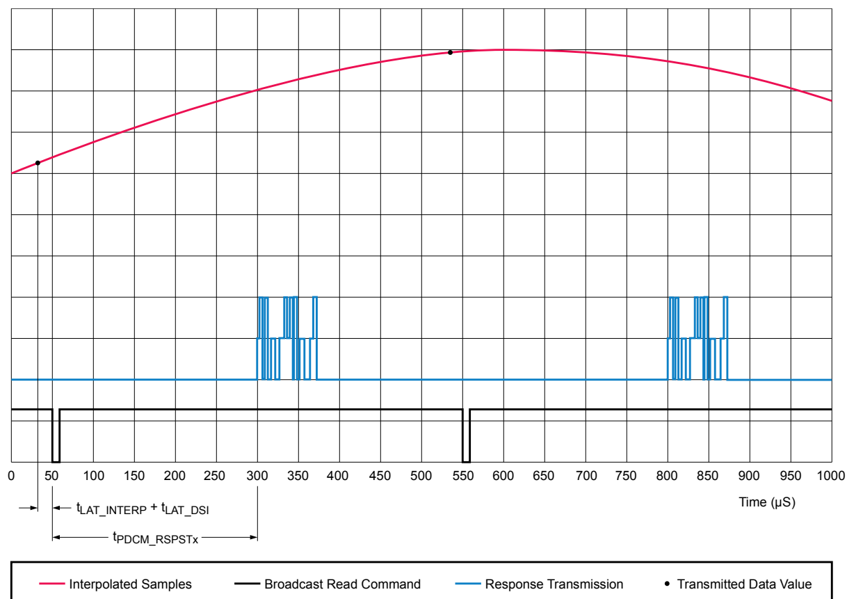
Figure 40. Simultaneous sampling mode
