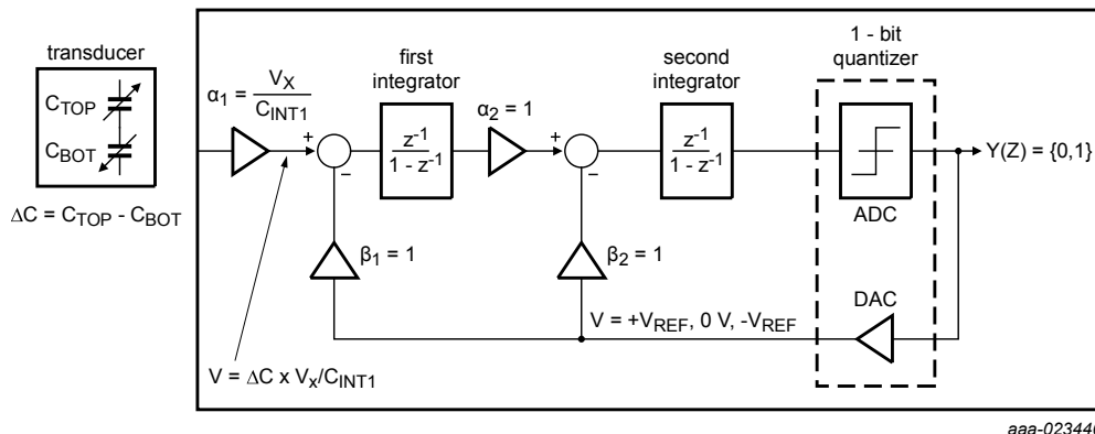
Figure 12. \Sigma\Delta converter block diagram
