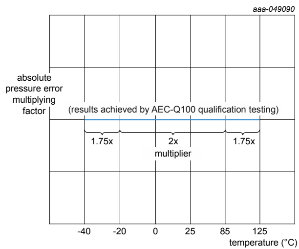
Figure 23. Absolute pressure accuracy multiplier over life
