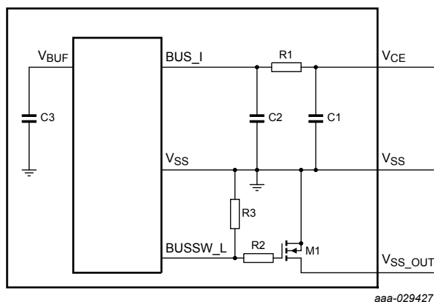
Figure 58. PSi5 daisy chain mode application diagram
