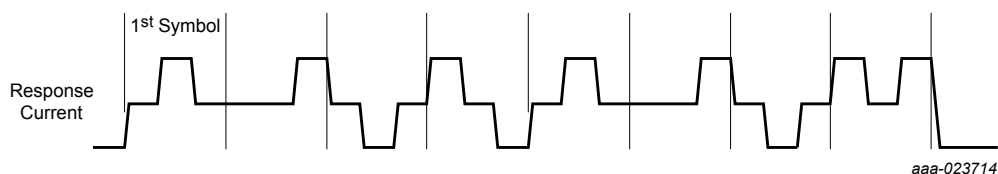
Figure 33. Command and response mode response example
