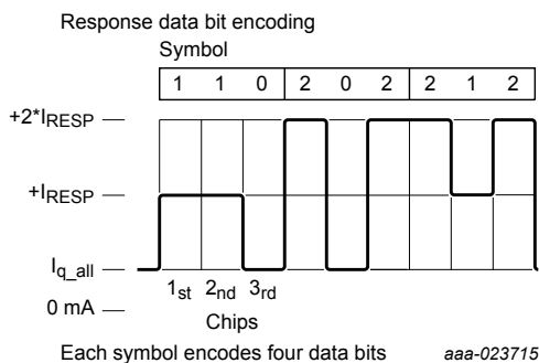
Figure 34. Response symbol encoding
