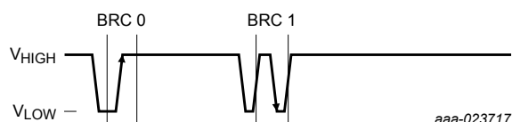
Figure 36. Background diagnostic mode command bit encoding
