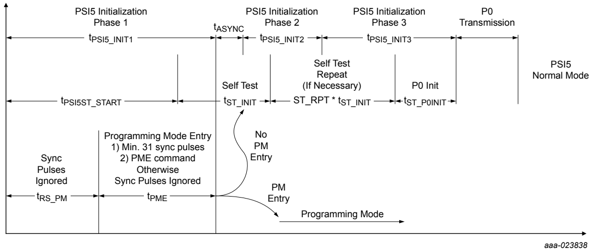
Figure 52. PSI5 initialization timing, asynchronous mode
