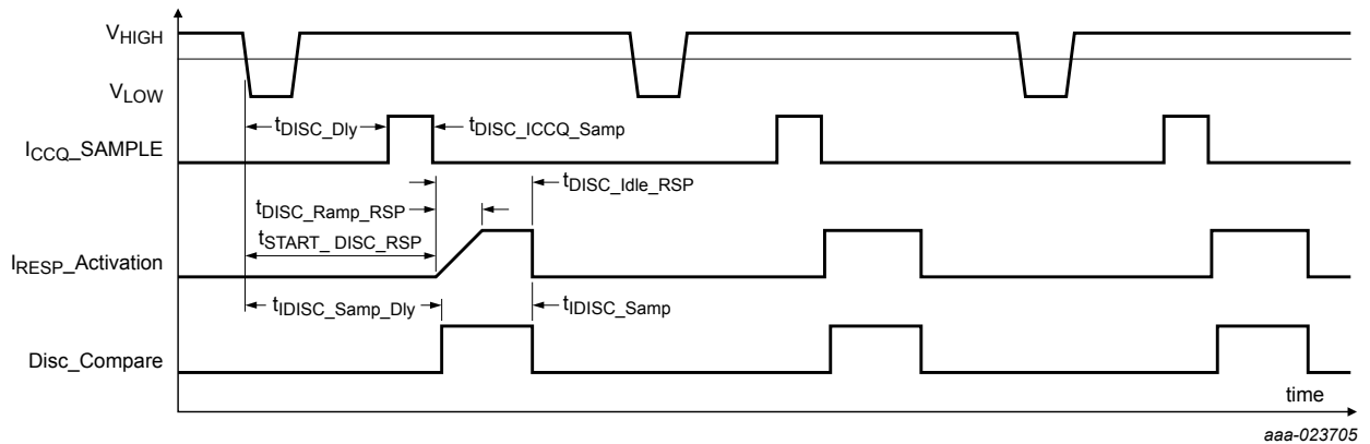
Figure 29. DSI3 discovery mode sensing timing diagram
