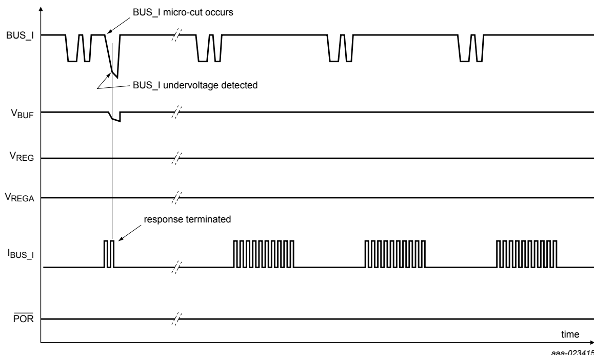
Figure 7. BUS_I micro-cut response (DSI3 or PSI5)
