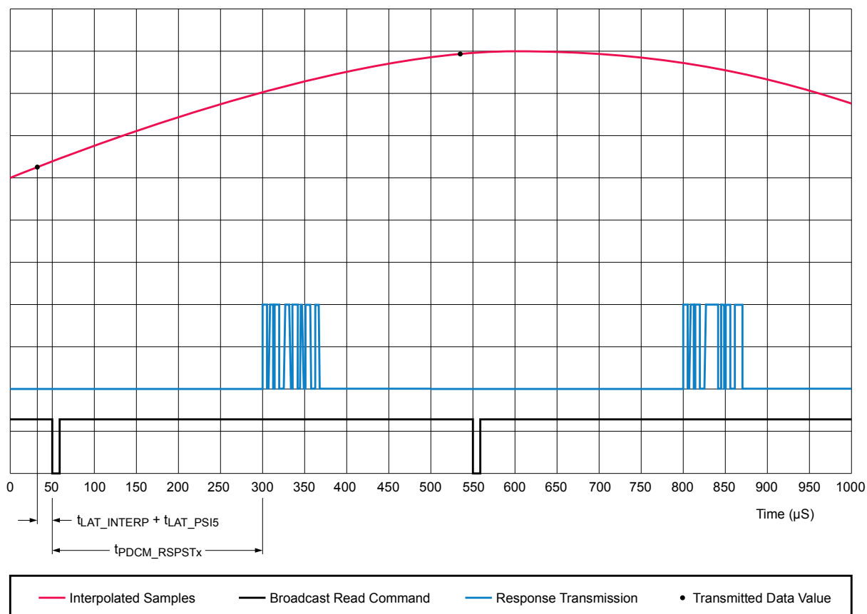
Figure 53. Simultaneous sampling mode
