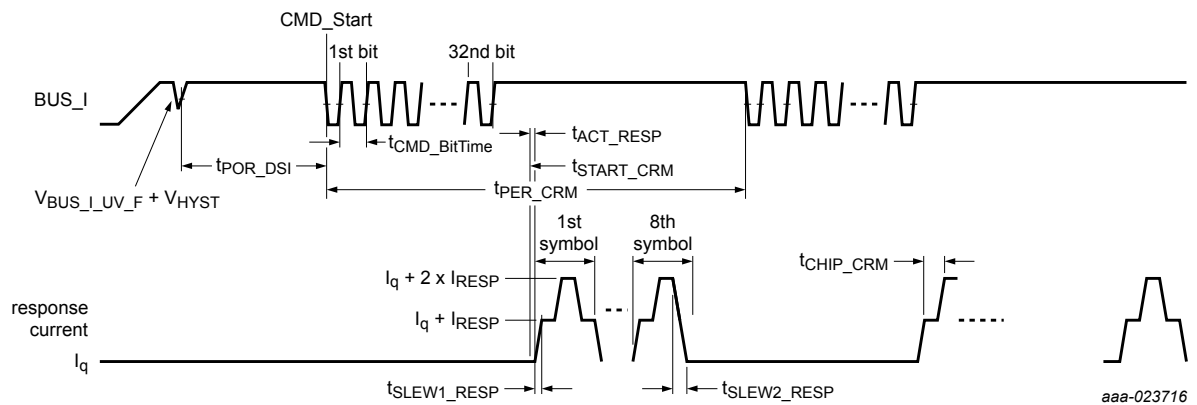
Figure 35. Command and response mode timing diagram
