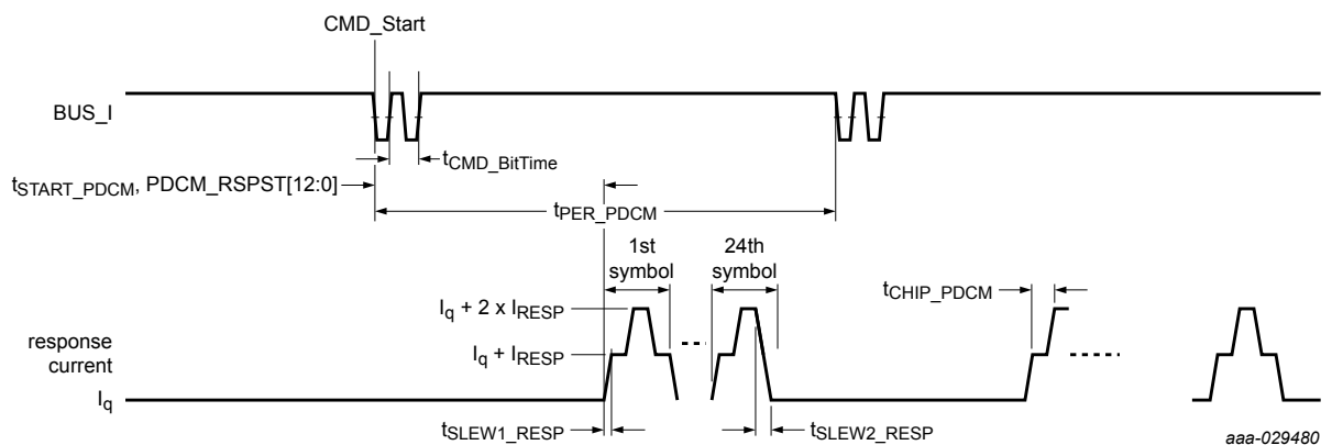
Figure 38. Periodic data collection mode timing diagram
