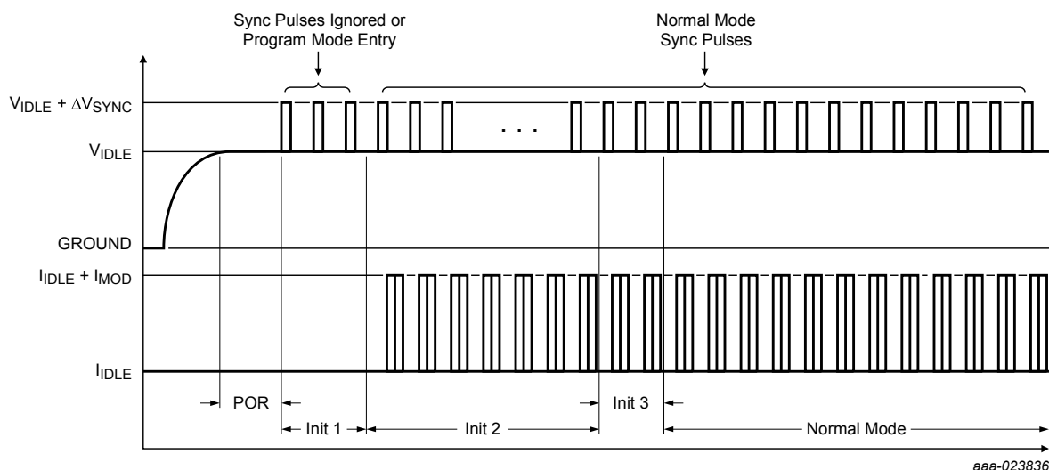
Figure 50. PSI5 sensor 10-bit initialization
