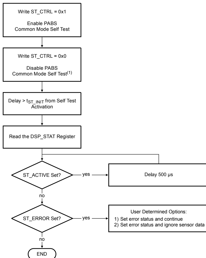
Figure 11. User-controlled PABS common mode self-test flowchart
