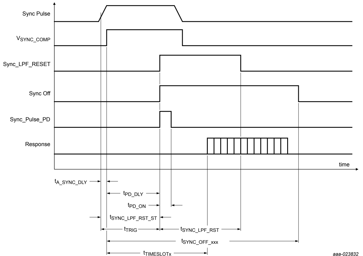
Figure 46. Synchronization pulse detection timing
