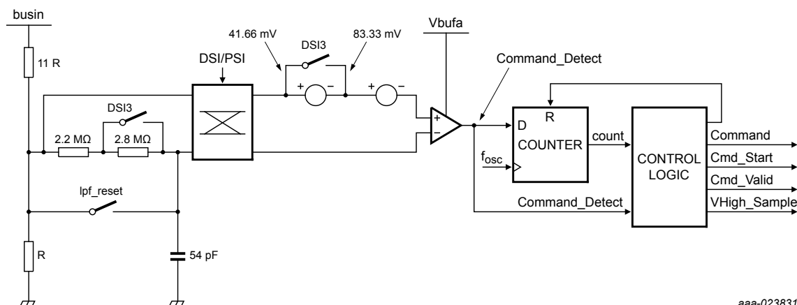
Figure 45. Synchronization pulse detection circuit
