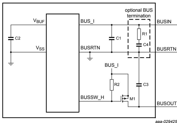
Figure 56. DSI3 switch connected daisy chain application diagram
