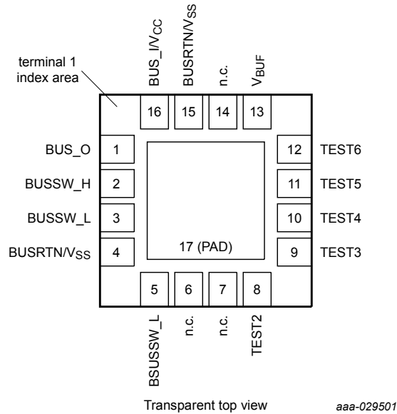
Figure 2. Pin configuration for HQFN16
