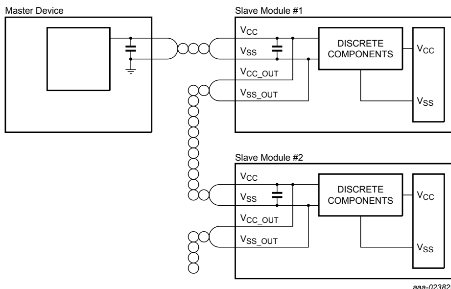
Figure 43. PSI5 satellite interface diagram
