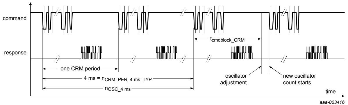
Figure 8. Command and response mode oscillator training timing diagram
