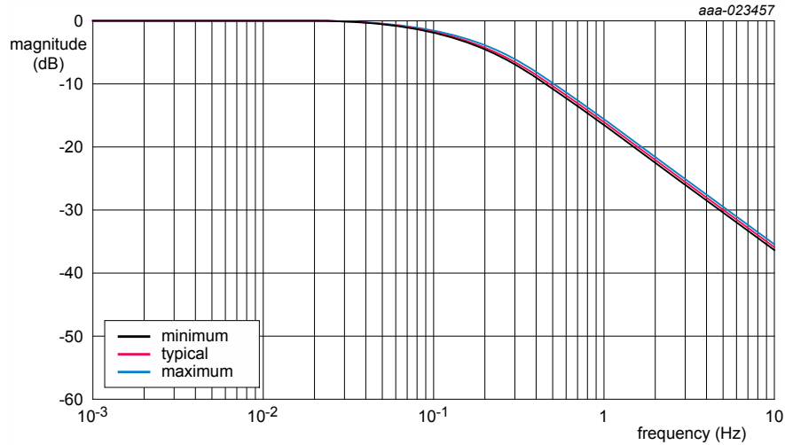
Figure 17. 0.16 Hz, 1-Pole P_0 low-pass filter response
