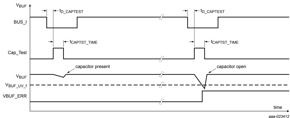
Figure 4. V_{BUF} capacitor monitor timing, DSI3
