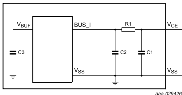
Figure 57. PSi5 parallel or universal mode application diagram
