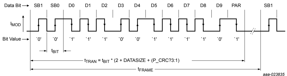
Figure 49. Example Manchester encoded data transfer – psi5-x10x
