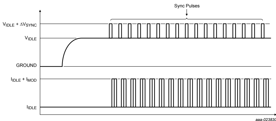
Figure 44. Synchronous communication overview
