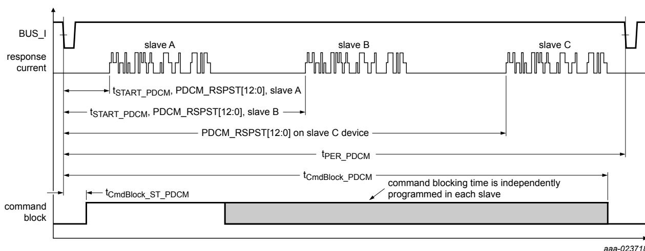
Figure 37. Periodic data mode response transmission
