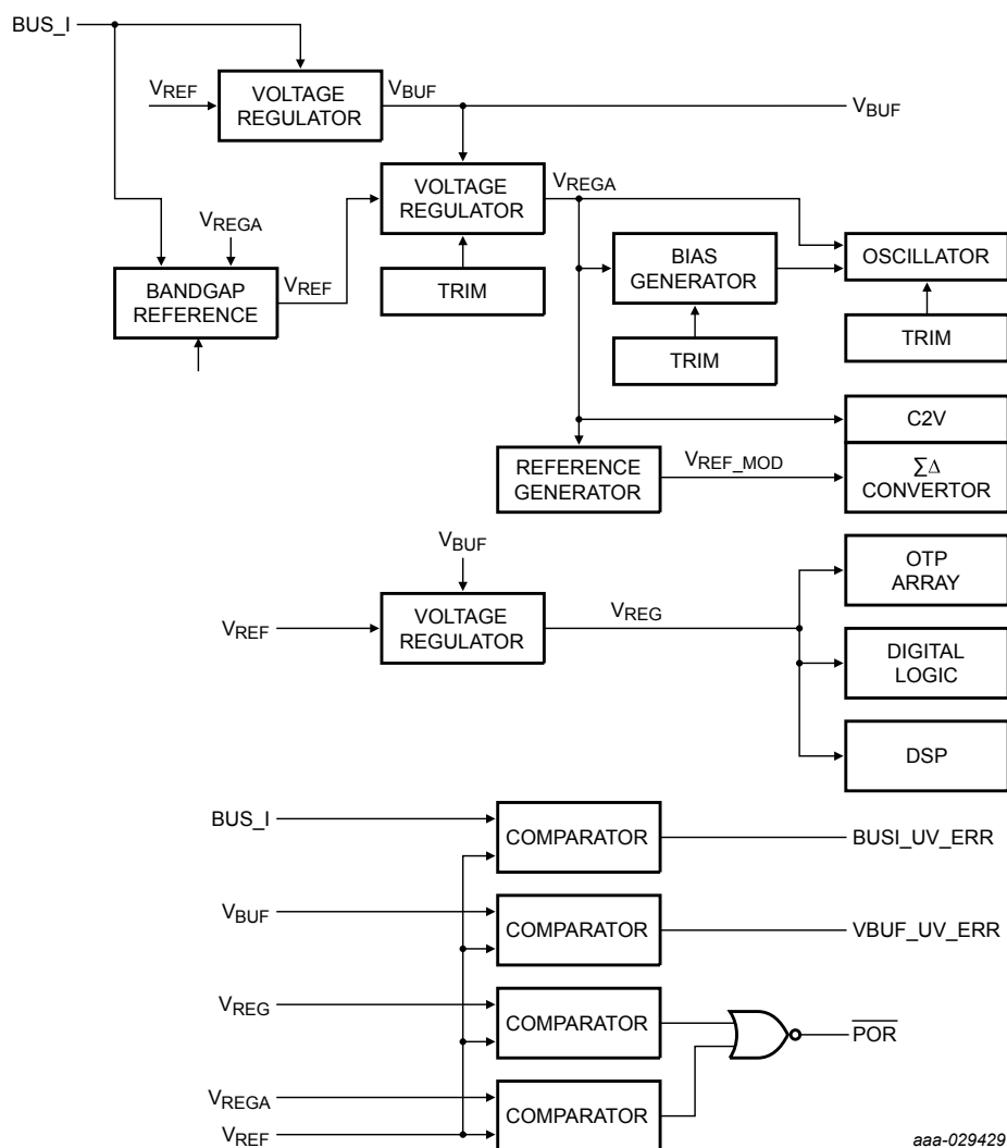
Figure 3. Voltage regulation and monitoring
