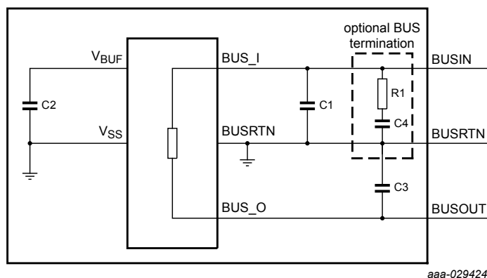
Figure 55. DSI3 discovery mode application diagram
