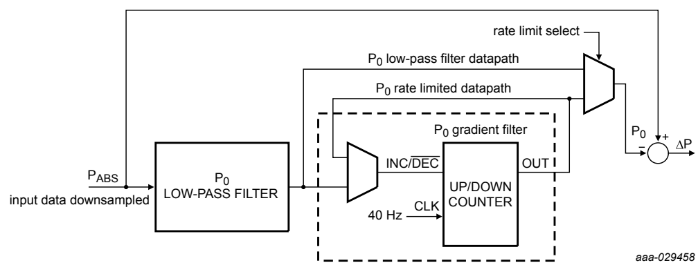
Figure 16. P_0 low-pass filter block diagram
