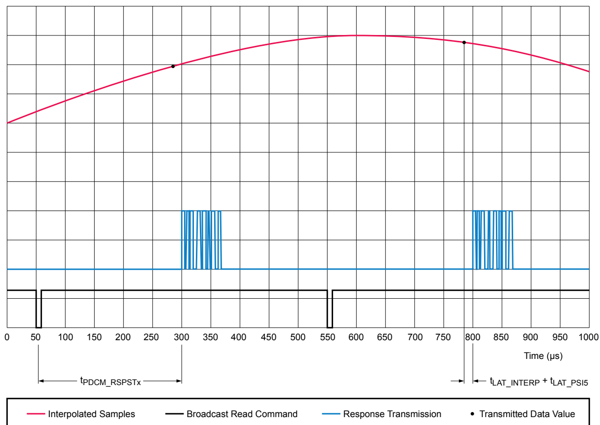
Figure 54. Synchronous sampling mode with minimum latency
