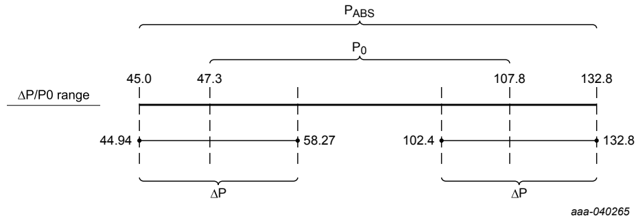
Figure 18. P_0 and P_{ABS} range
