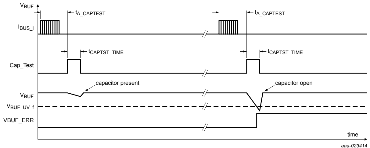
Figure 6. V_{BUF} capacitor monitor timing, PSI5 asynchronous mode
