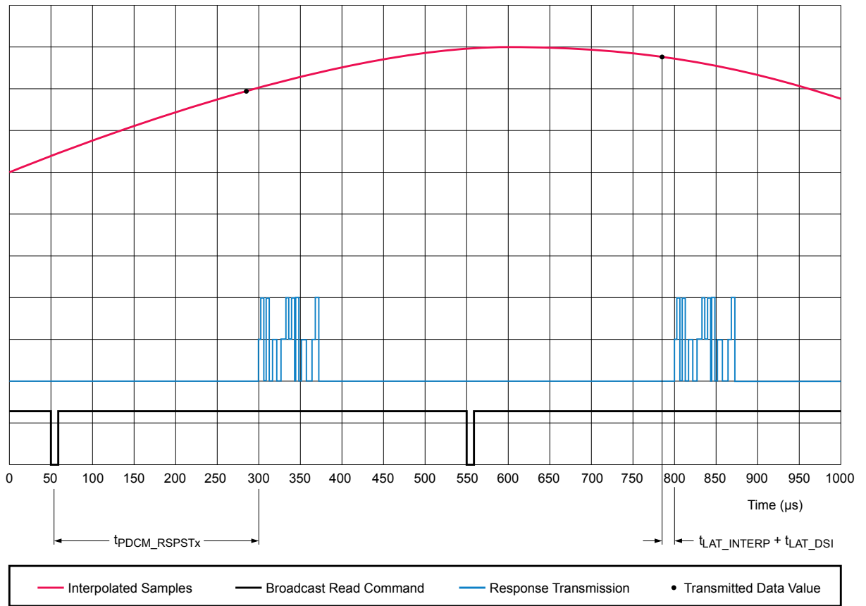
Figure 41. Synchronous sampling mode with minimum latency
