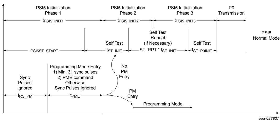
Figure 51. PSI5 initialization timing, synchronous mode
