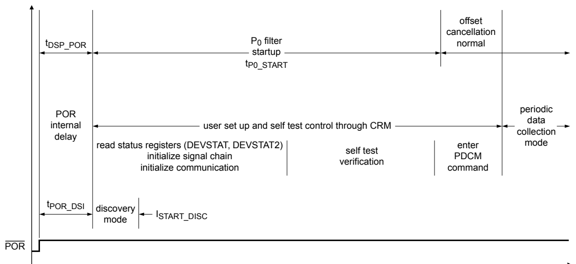
Figure 42. Initialization timing
