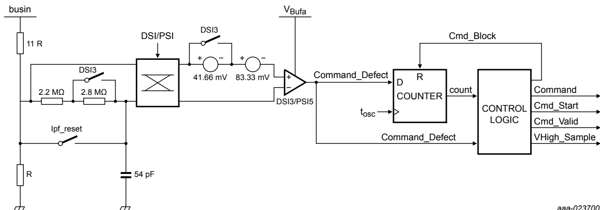
Figure 24. Command receiver physical layer
