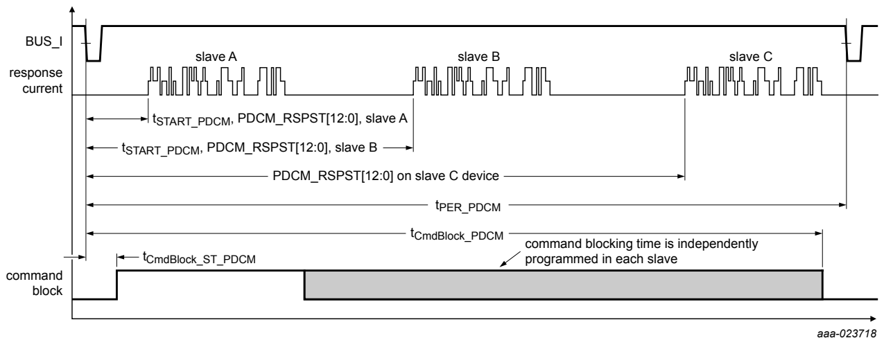
Figure 10. PSI5 oscillator training timing diagram
