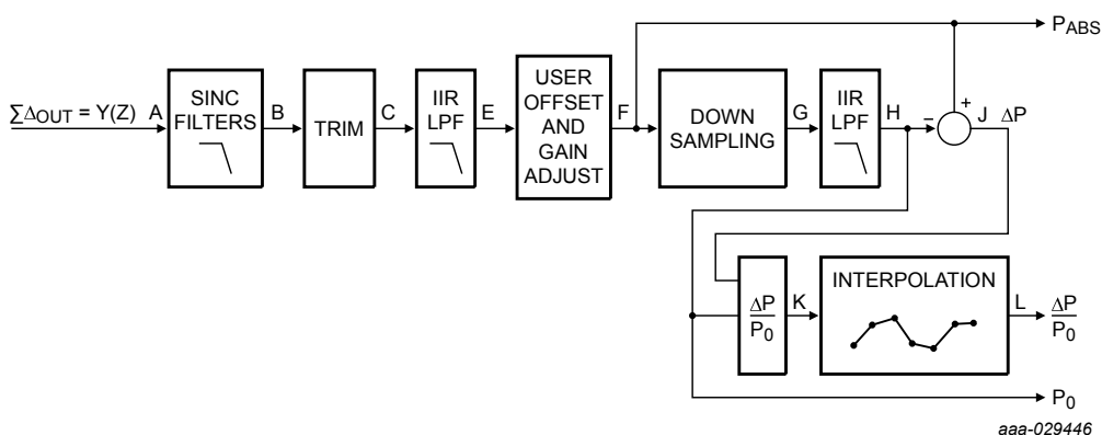
Figure 13. Signal chain diagram
