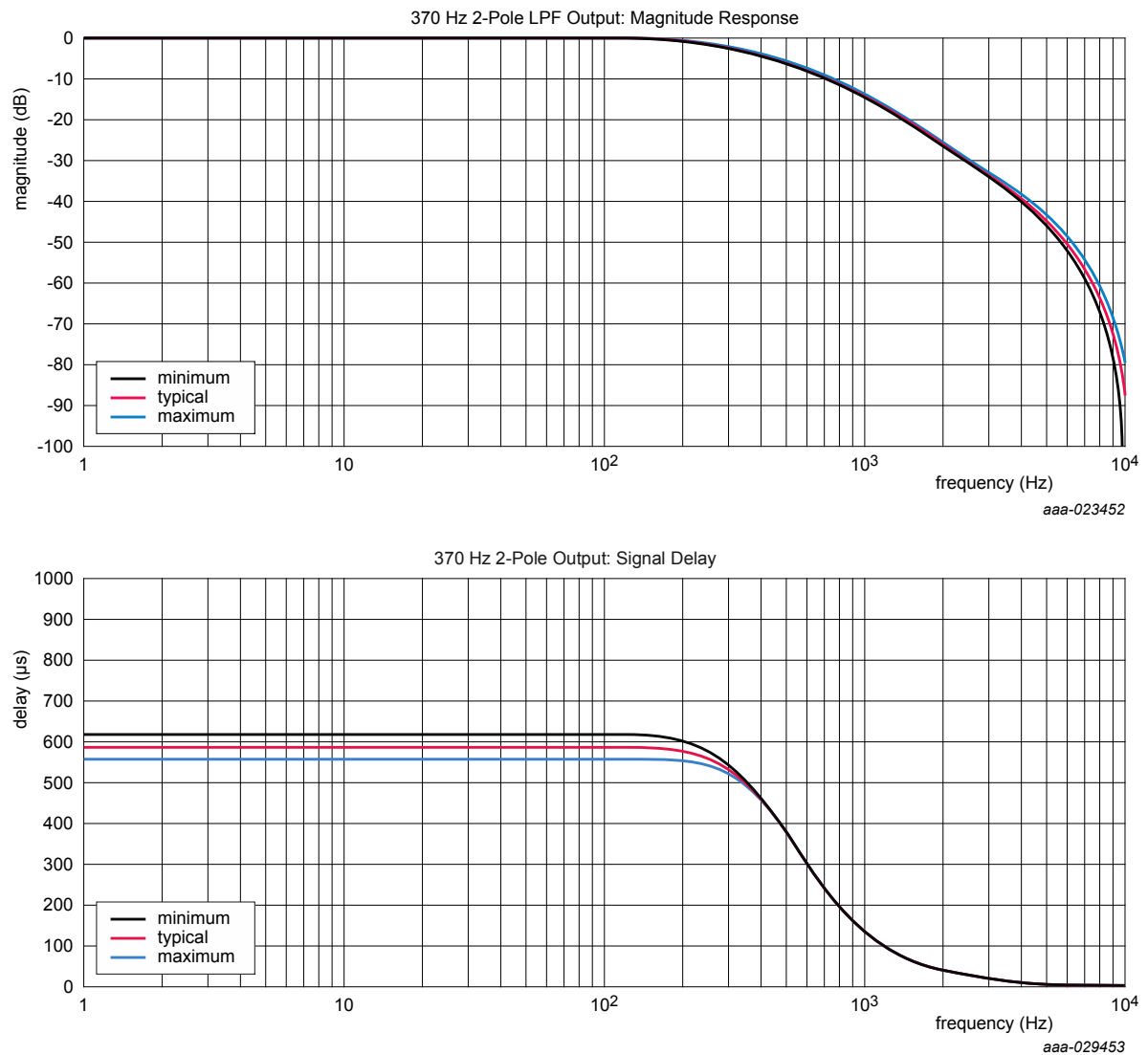
Figure 15. 370 Hz, 2-pole low-pass filter response
