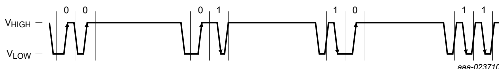
Figure 32. Command and response mode command bit encoding
