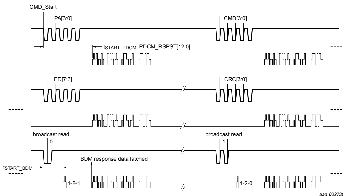
Figure 39. Background diagnostic mode timing diagram
