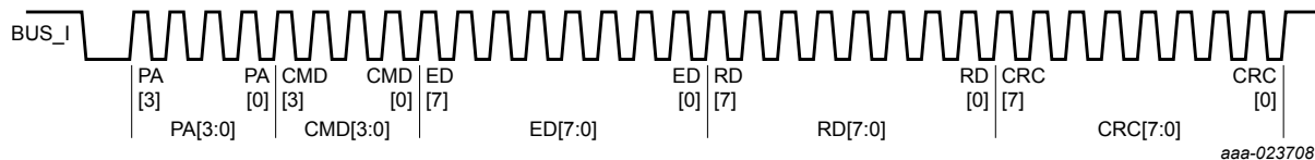
Figure 31. Command and response mode command example
