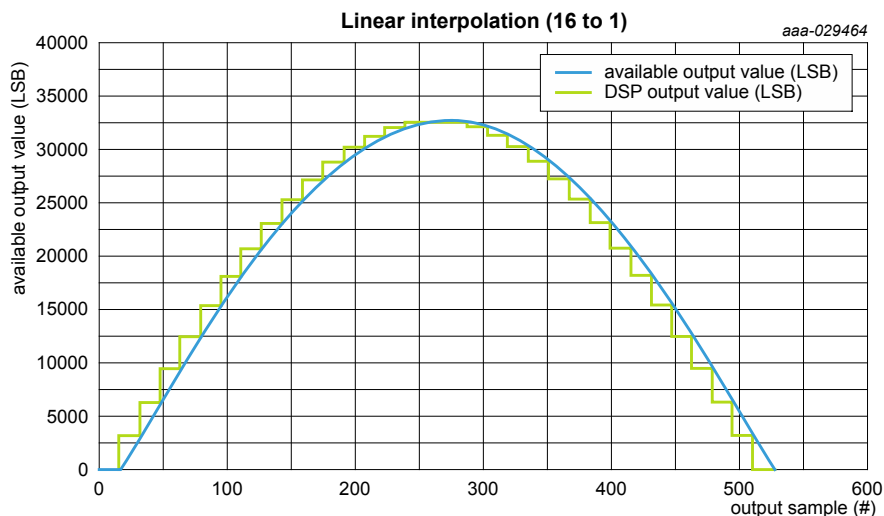
Figure 19. Output interpolation example
