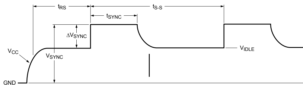
Figure 47. Sync pulse characteristics
