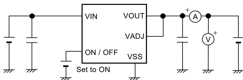
Figure 13 Test Circuit 8
