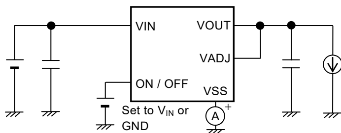
Figure 12 Test Circuit 7
