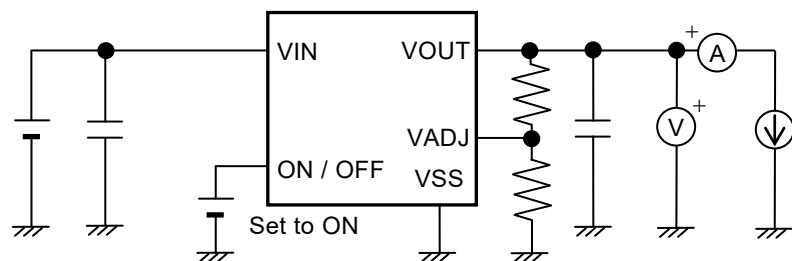
Figure 16 Test Circuit 11
