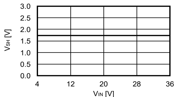
1. 12 High level input voltage ( V_{SH} ) vs. Input voltage ( V_{IN} )
