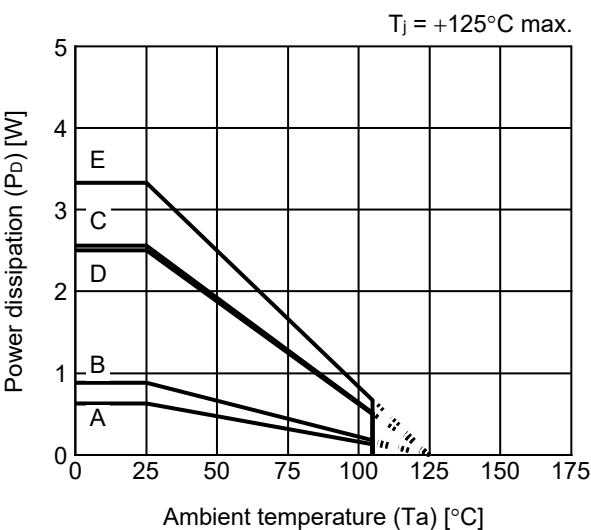
HTMSOP-8
