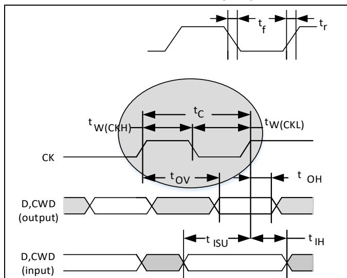
Figure 24. SD default mode
