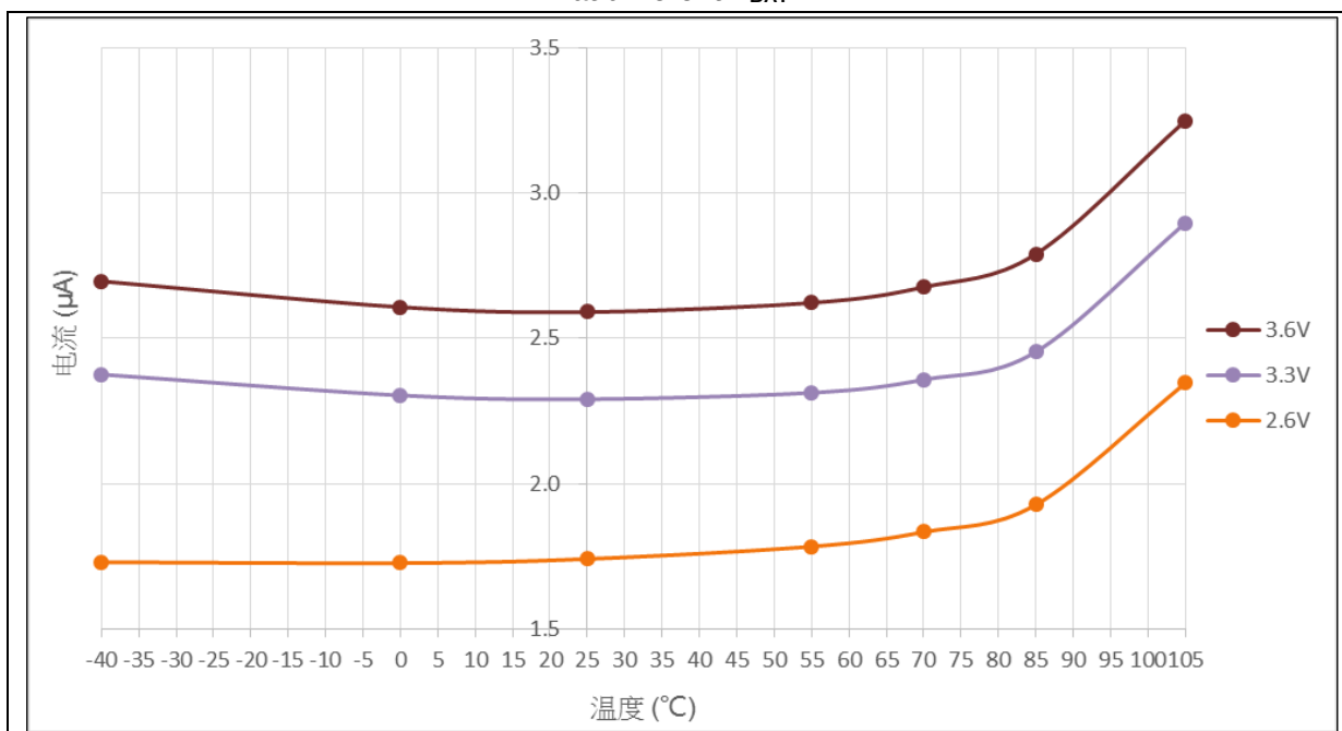
Figure 11. Typical current consumption on V_{BAT} with LEXTR and RTC ON vs. temperature at different V_{BAT}
