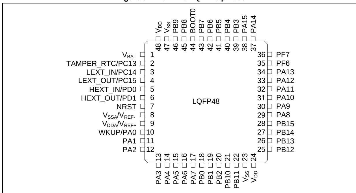
Figure 3. AT32F413 LQFP48 pinout
