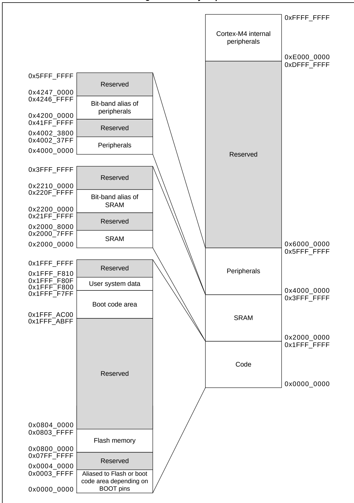
Figure 6. Memory map
