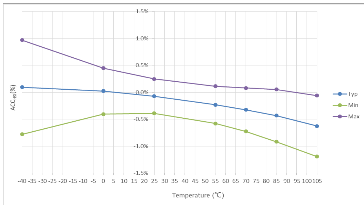
Figure 17. HICK clock frequency accuracy vs. temperature
