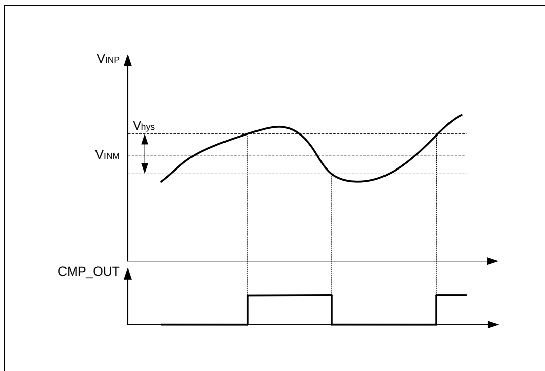
Figure 30. CMP hysteresis
