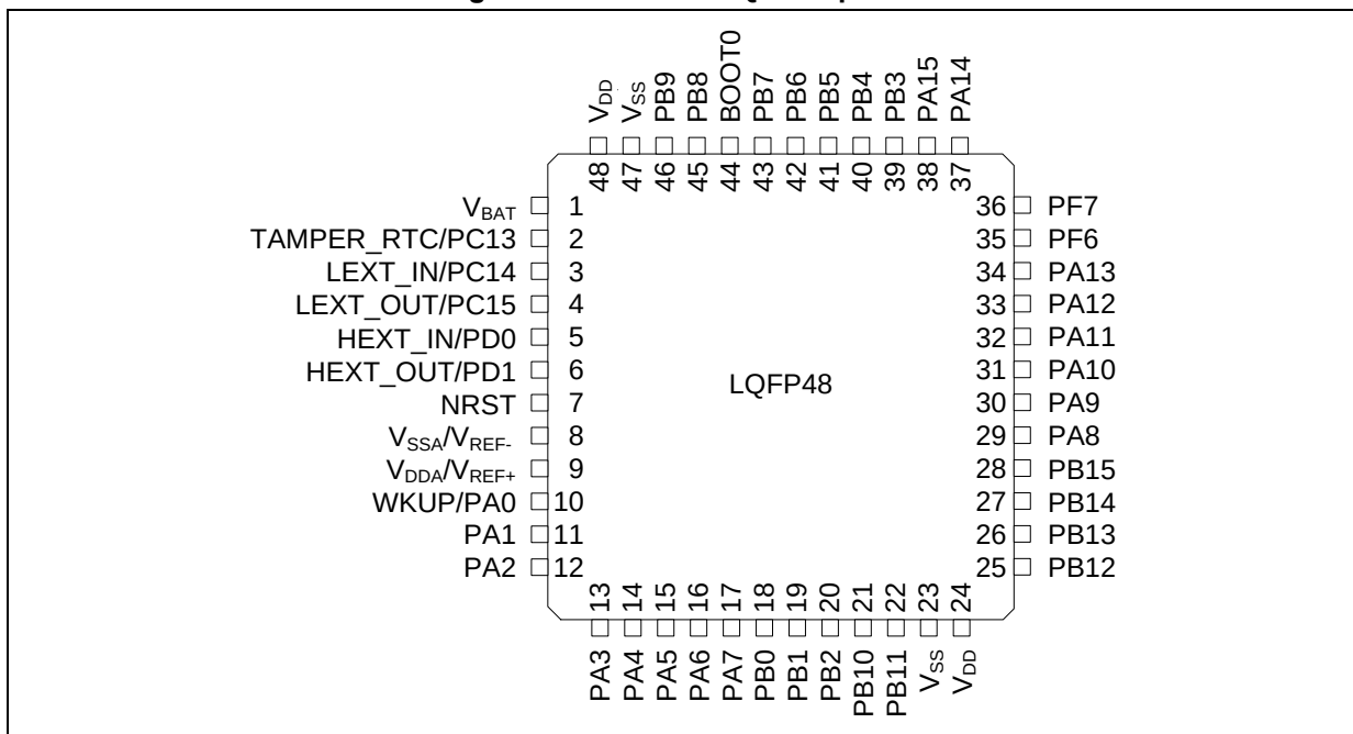
Figure 3. AT32F415 LQFP48 pinout
