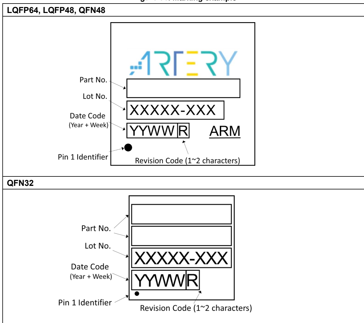
Figure 36. Marking example
