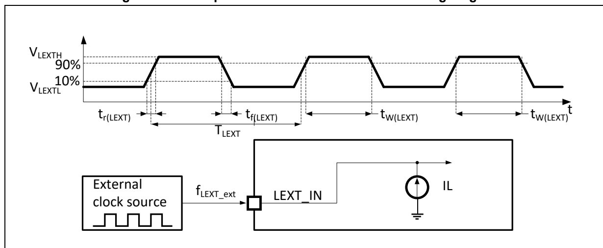
Figure 17. Low-speed external clock source AC timing diagram
