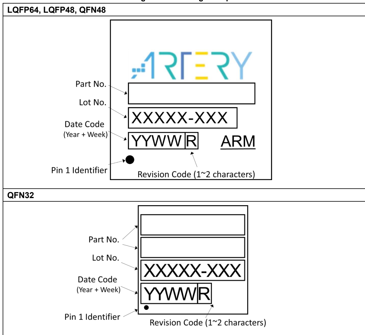
Figure 35. Marking example
