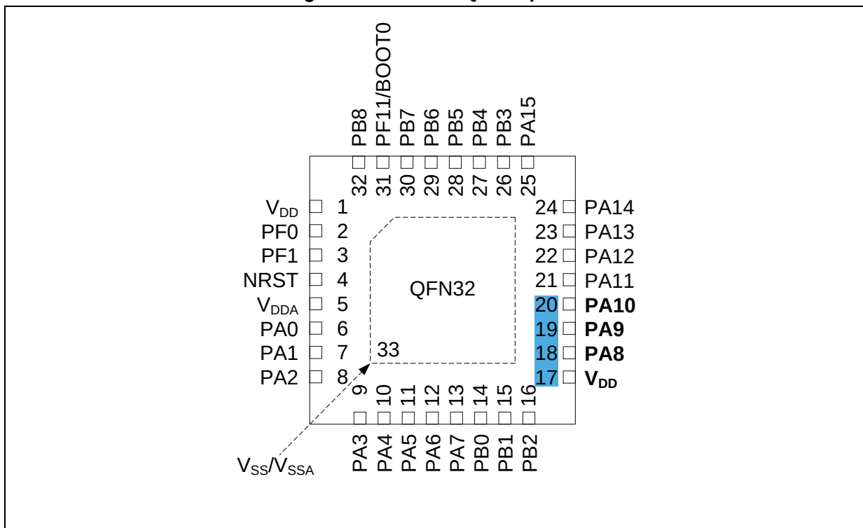
Figure 8. AT32F402 QFN32 pinout
