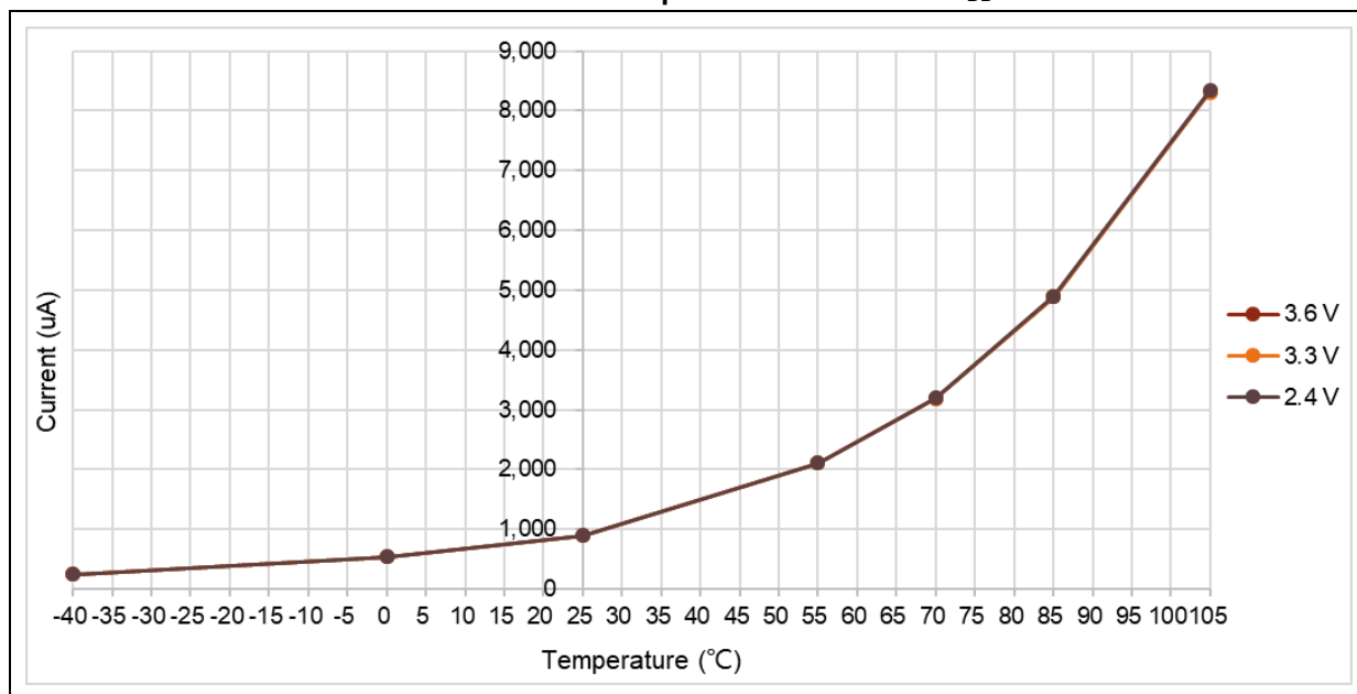
Figure 11. Typical current consumption in Deepsleep mode with LDO in run mode vs. temperature at different V DD
