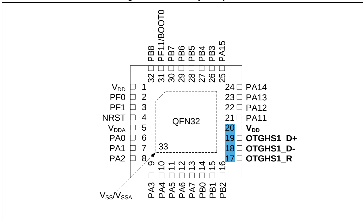
Figure 7. AT32F405 QFN32 pinout
