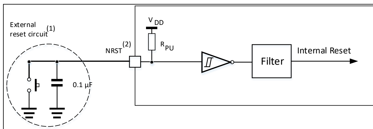
Figure 39. Recommended NRST pin protection
