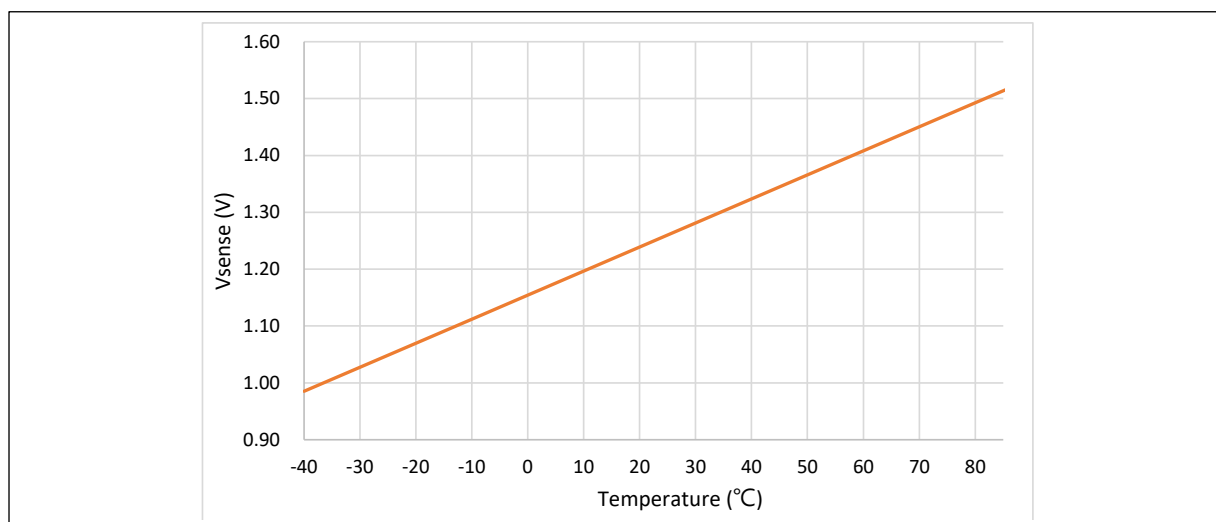
Figure 53. V_{SENSE} versus temperature
