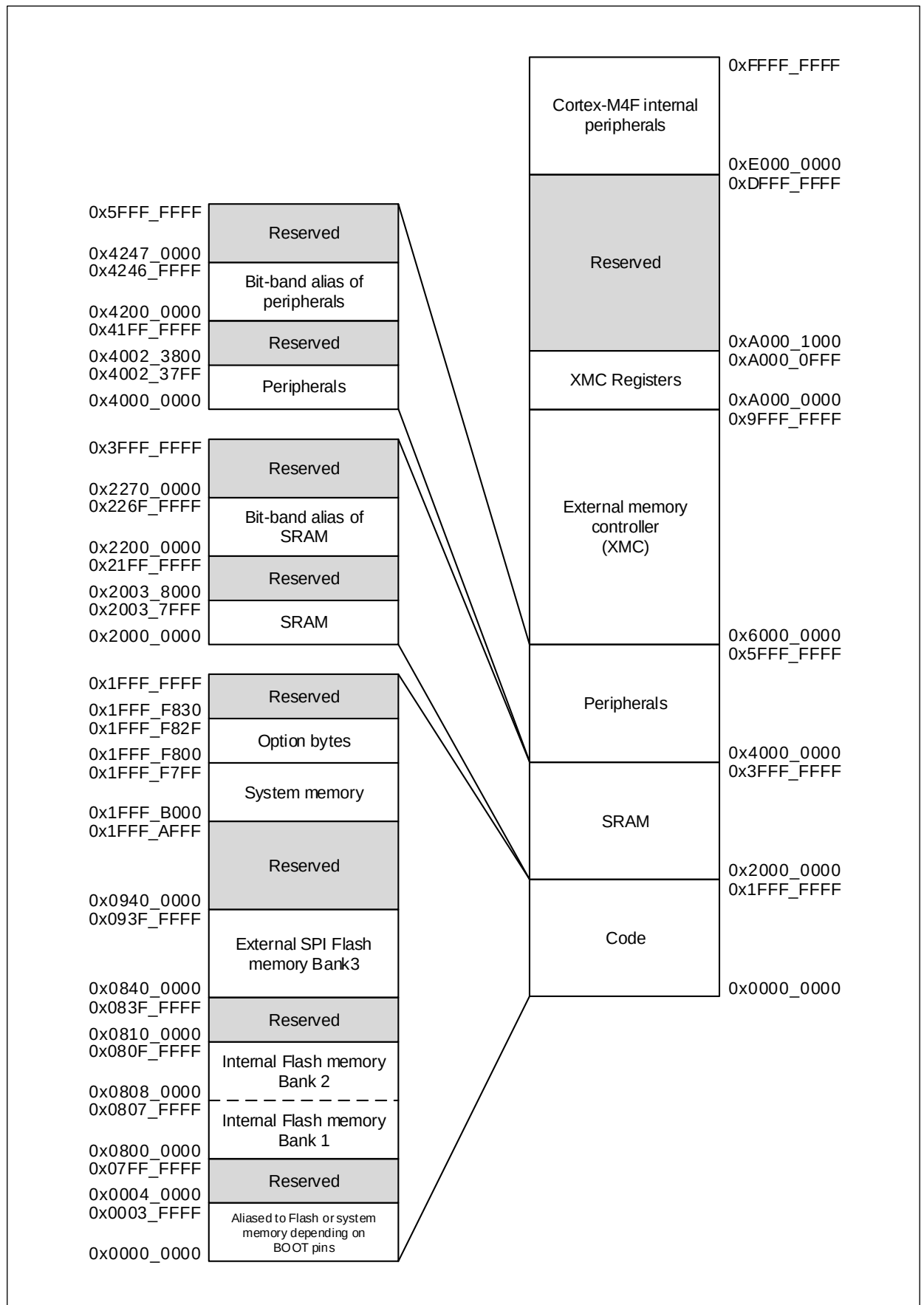
Figure 8. Memory map
