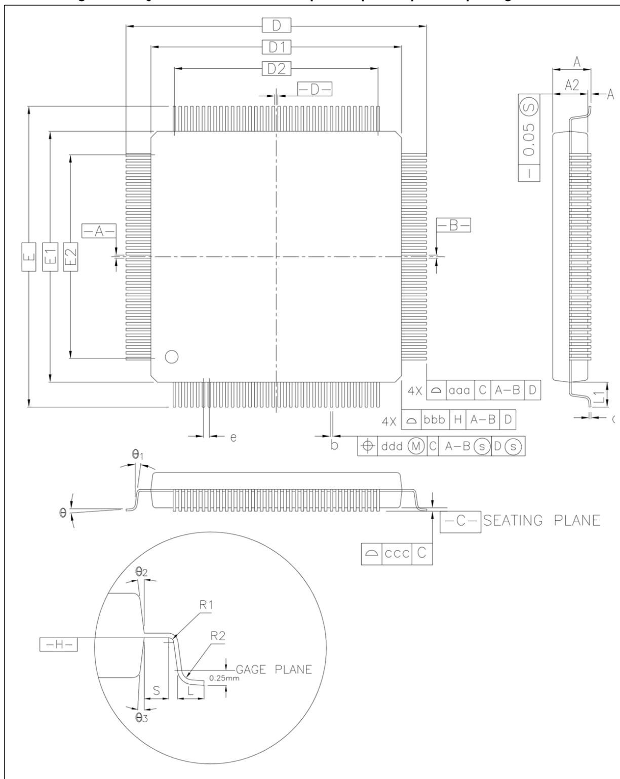
Figure 54. LQFP144 – 20 x 20 mm 144 pin low-profile quad flat package outline
