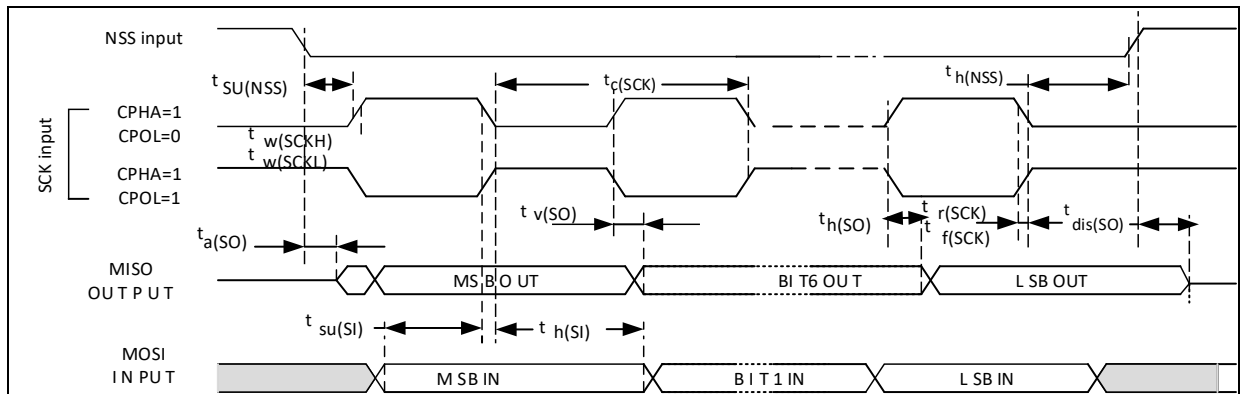
Figure 42. SPI timing diagram - slave mode and CPHA = 1 (1)
