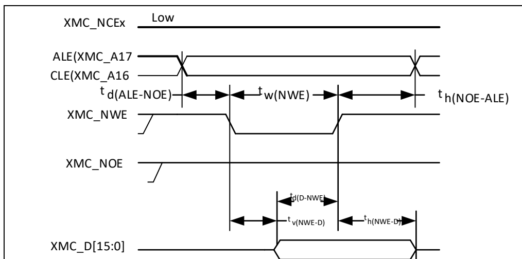
Figure 38. NAND controller waveforms for common memory write access
