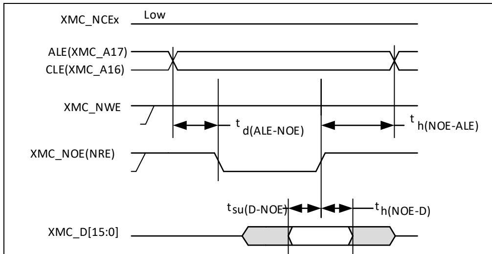
Figure 35. NAND controller waveforms for read access
