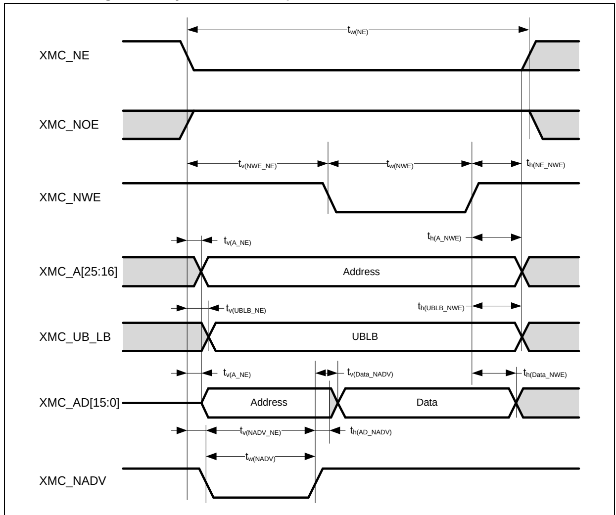
Figure 17. Asynchronous multiplexed PSRAM / NOR write waveforms
