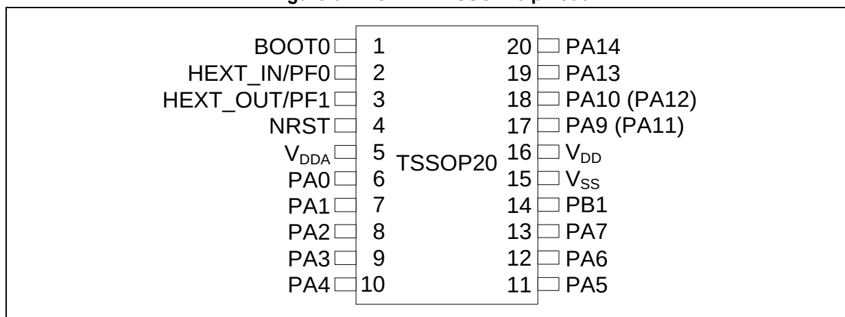
Figure 6. AT32F421 TSSOP20 pinout
