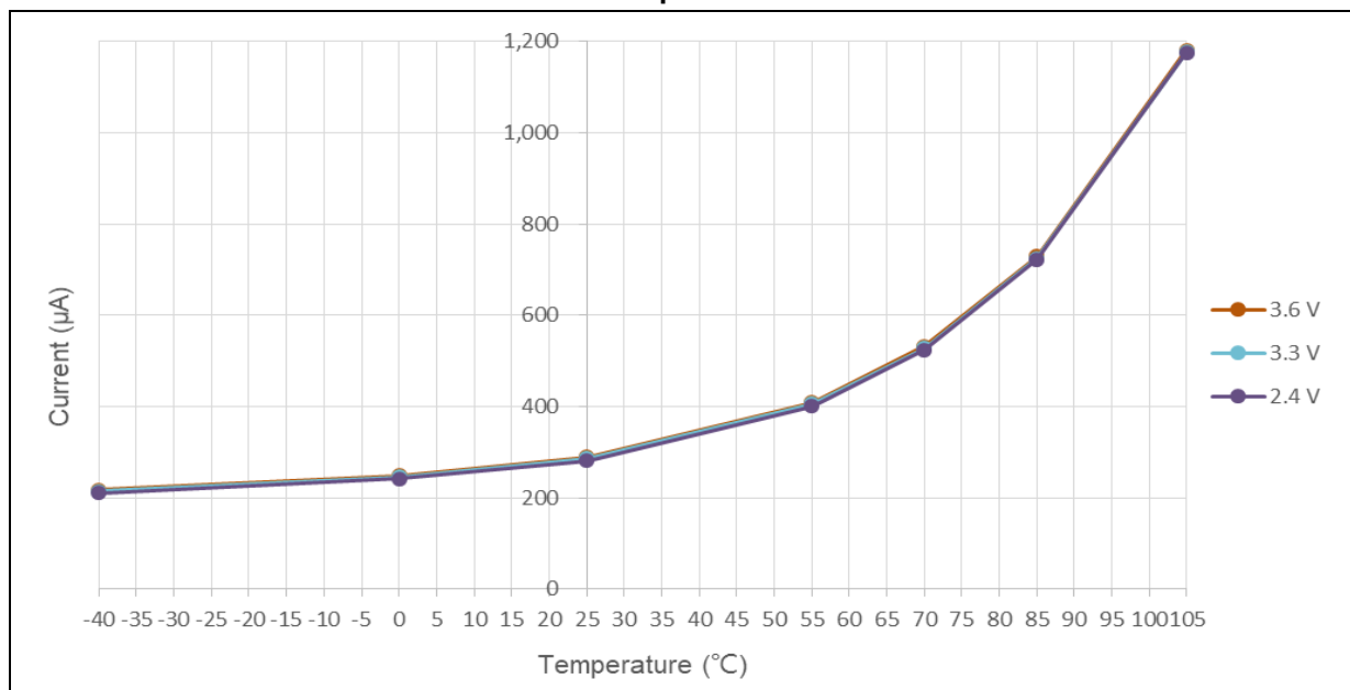
Figure 9. Typical current consumption in Deepsleep mode with LDO in run mode vs. temperature at different V DD
