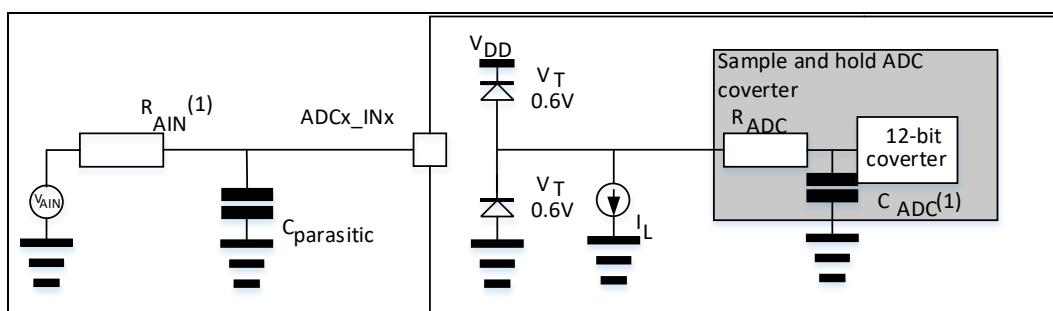
Figure 29. Typical connection diagram using the ADC
