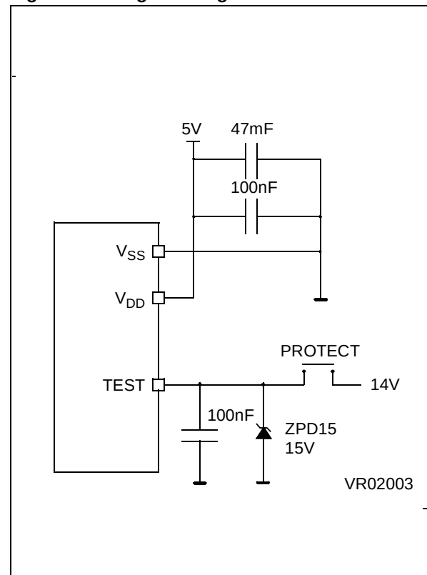
Figure 55. Programming Circuit
