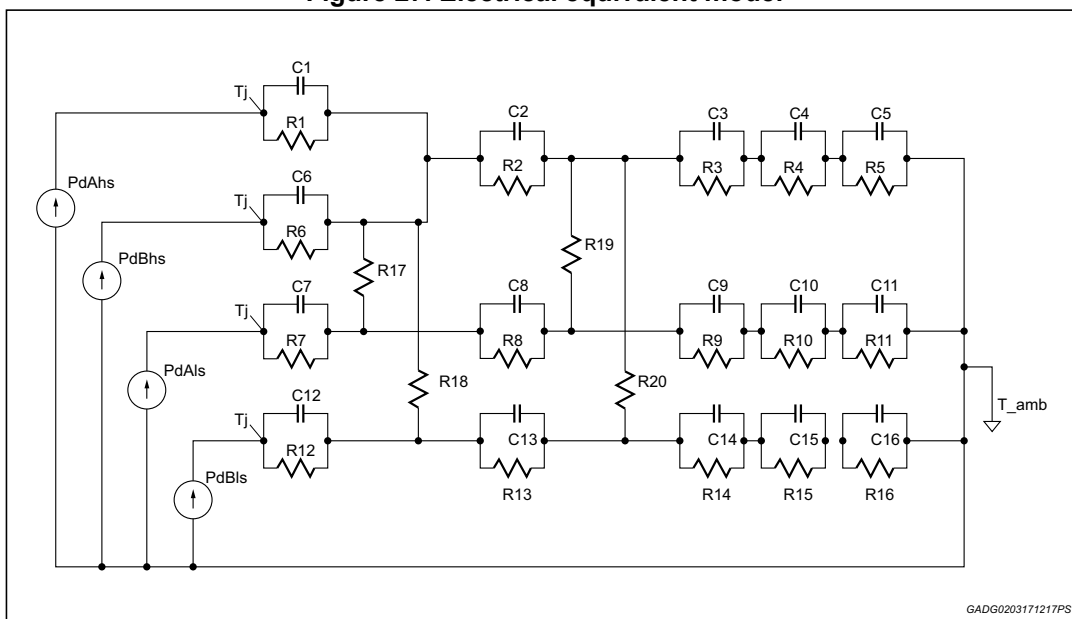
Figure 27. Electrical equivalent model
