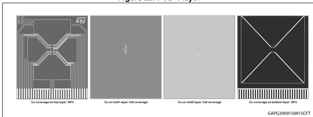
Figure 22. PCB 4 layer
