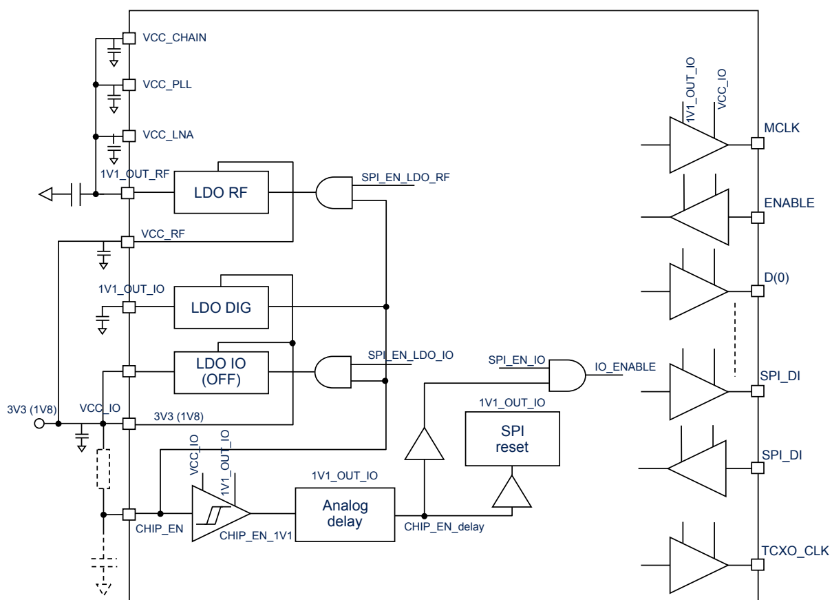
Figure 3. Power configuration
