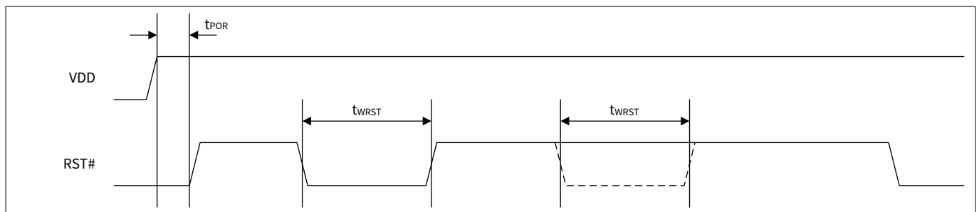
Figure 5 Reset timing
