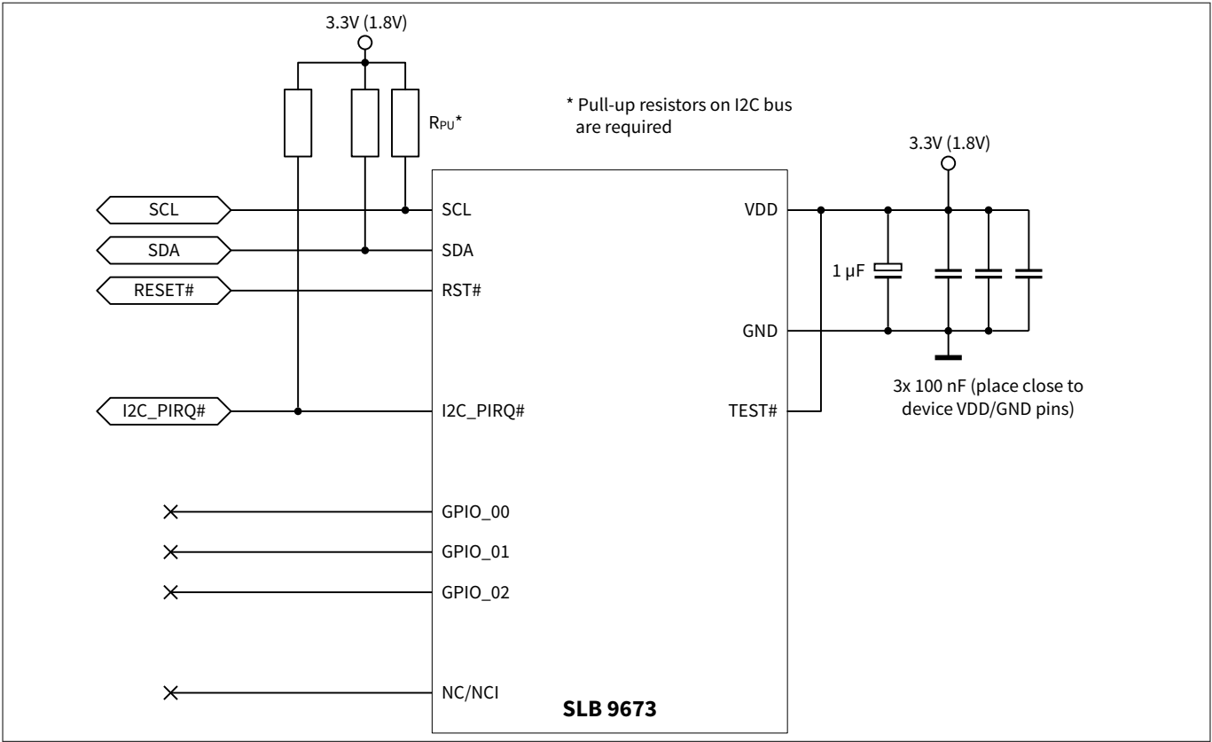
Figure 7 Typical schematic
