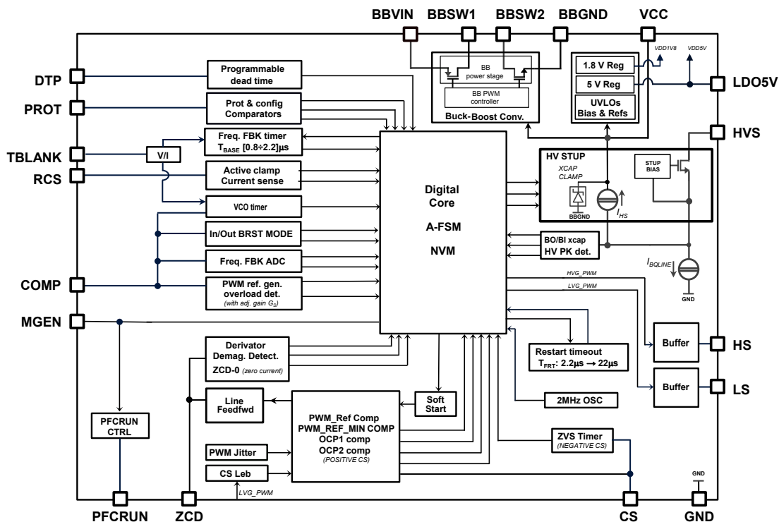
Figure 1. Block diagram
