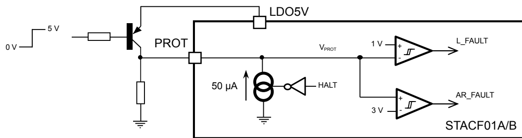
Figure 38. Remote ON/OFF function using the PROT pin: principle schematic
