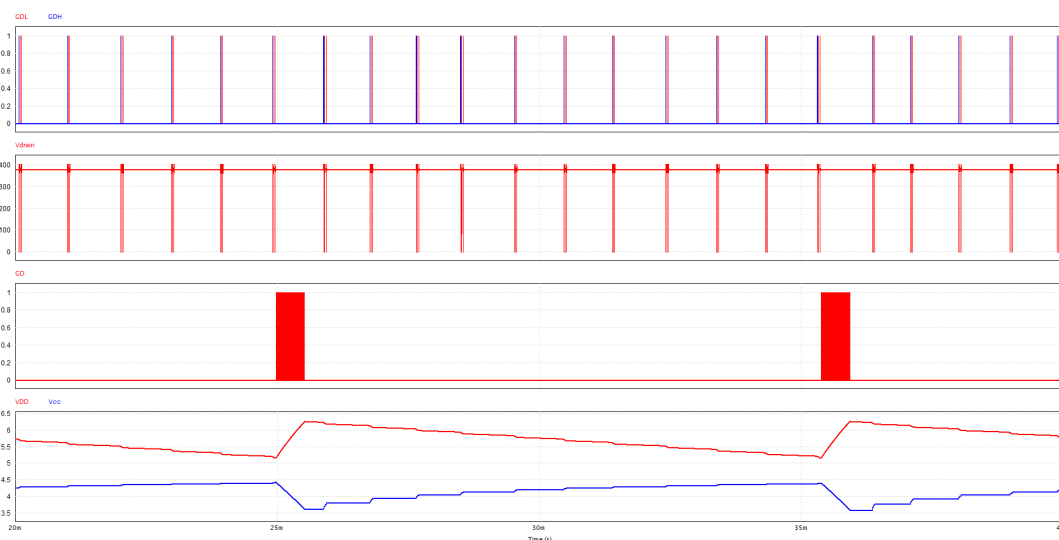
Figure 22. Auxiliary buck-boost operation during burst mode of main converter
