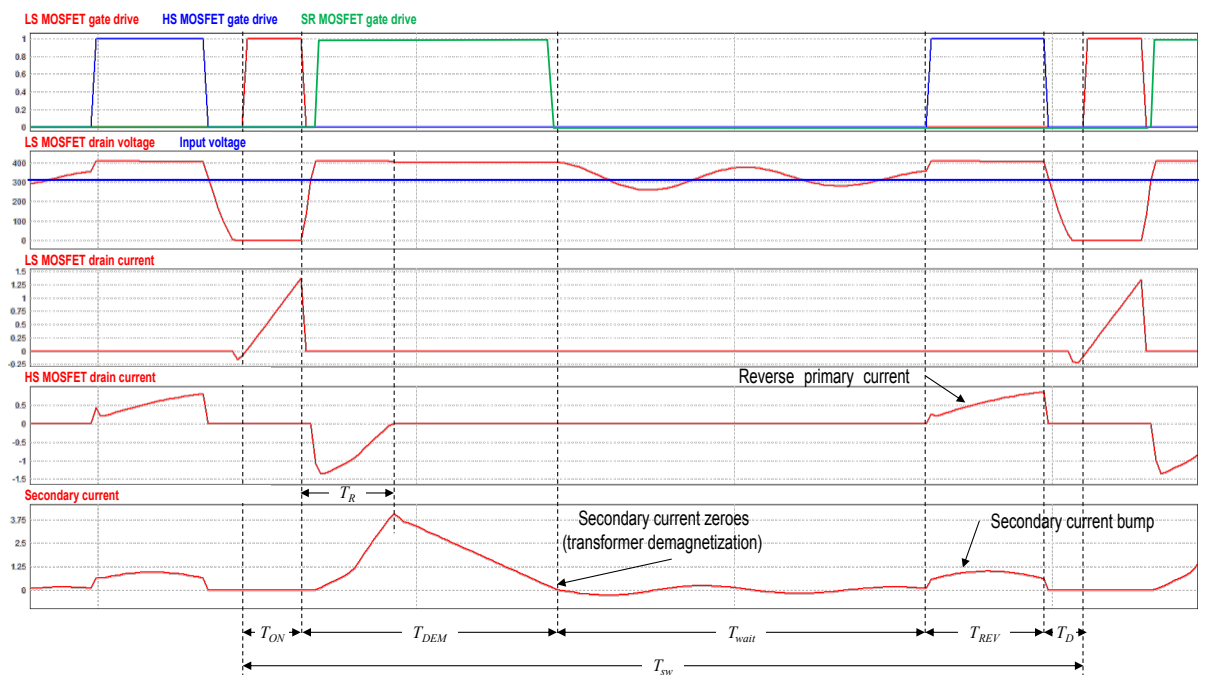
Figure 6. NC-ACF converter: DCM key waveforms (light load conditions)
