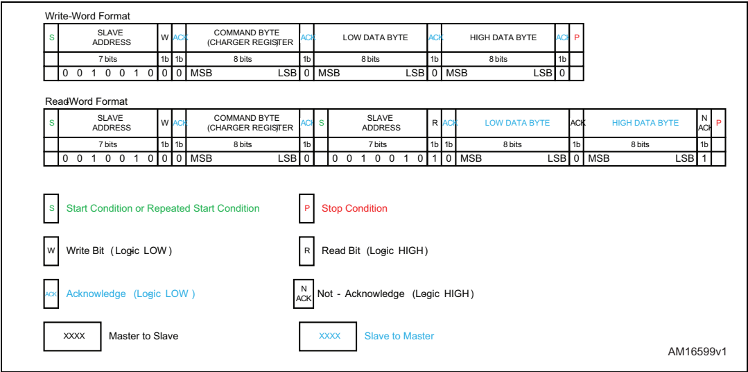
Figure 4. SMBus write-word and read-word protocols
