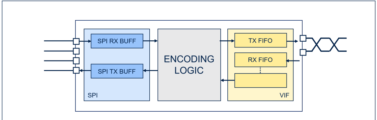
Figure 8. SPI – VIF interface management
