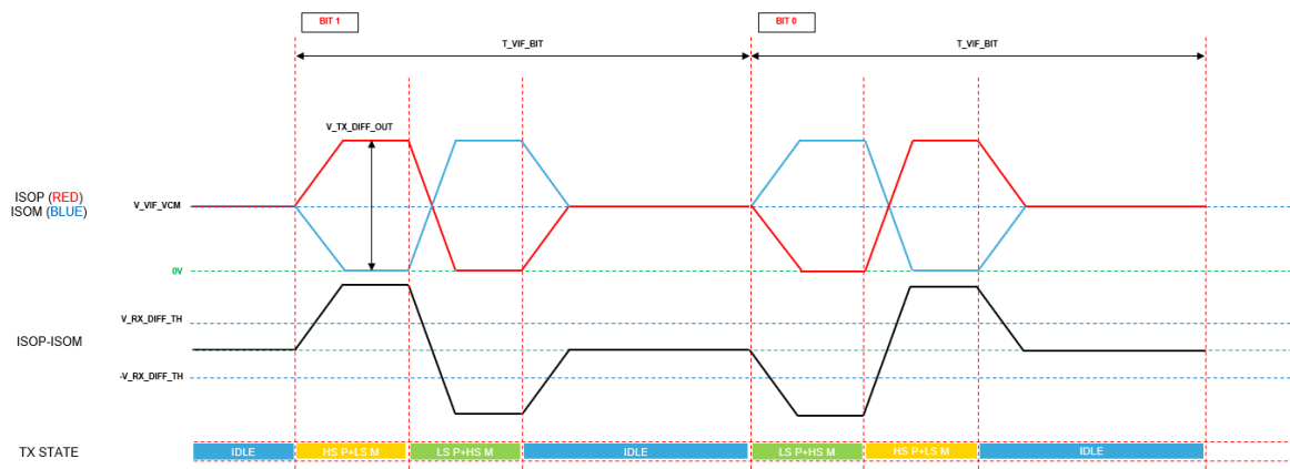
Figure 10. VIF waveform
