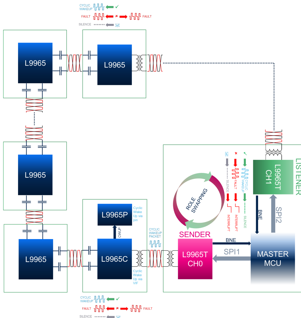
Figure 7. CYCLIC WAKEUP operation
