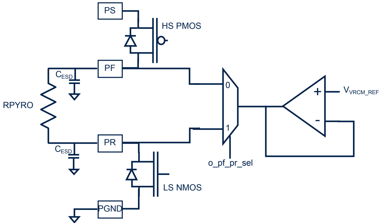
Figure 23. HS/LS deployment FETs test
