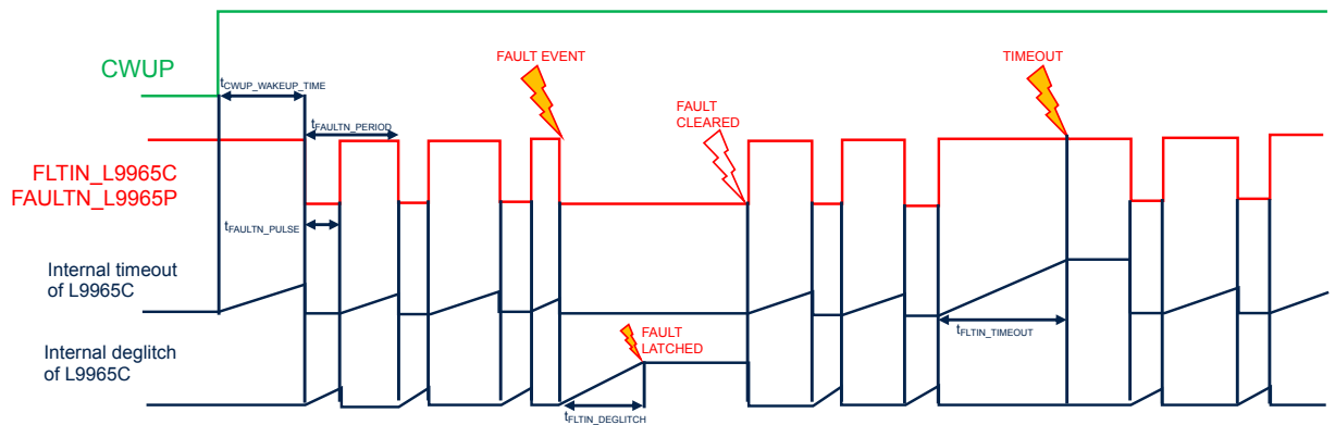
Figure 7. FAULTN cyclic pulse generation start
