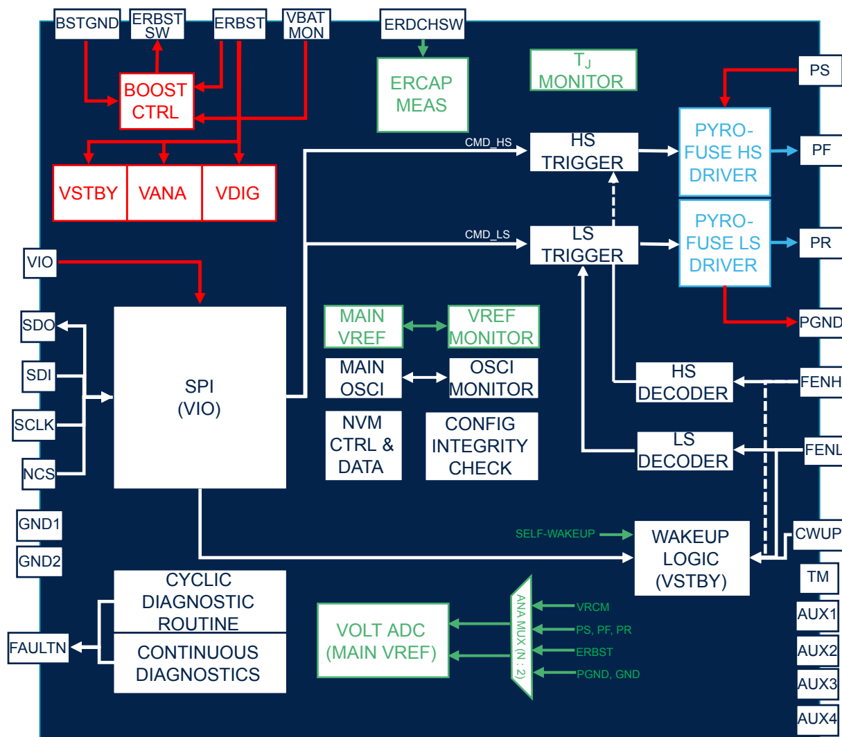
Figure 1. Block diagram
