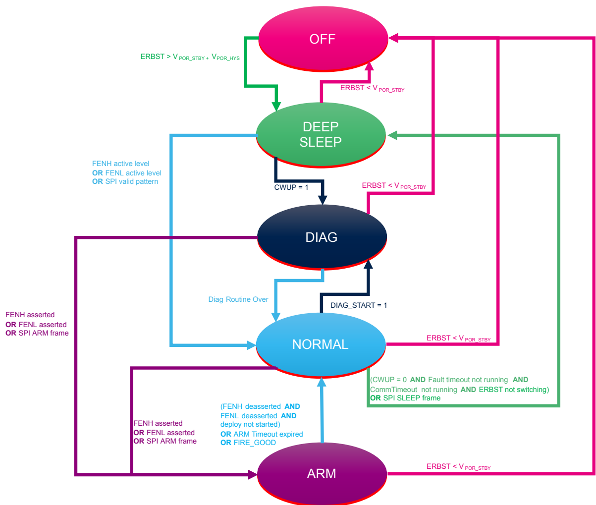
Figure 3. Device FSM
