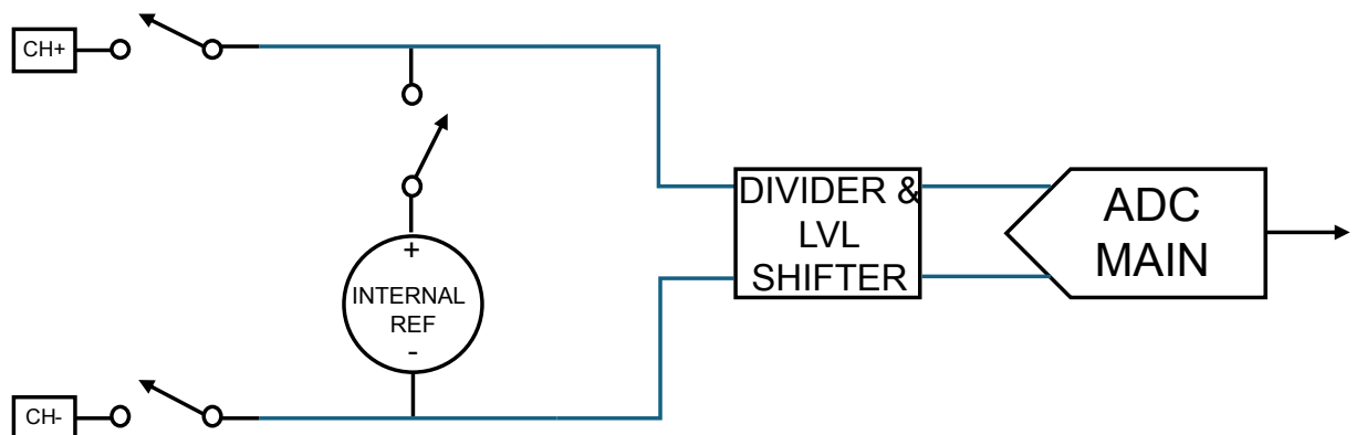
Figure 19. Differential ADC HWSC
