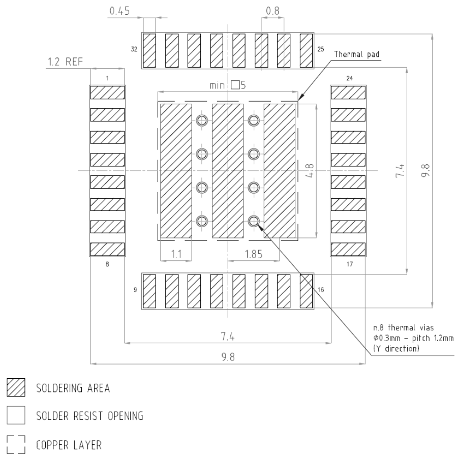
Figure 38. TQFP32L (7x7x1 mm 32+4L exposed pad down) pcb land pattern
