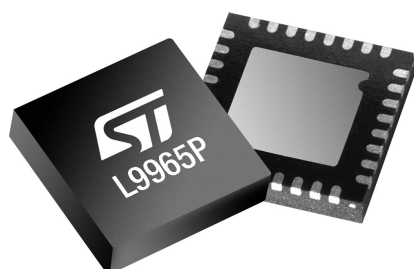
VFQFN32+4L 5x5x0.9 mm
