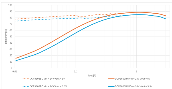
Figure 7. DCP3603B – Efficiency ( V_{IN} = 24\text{ V} )
