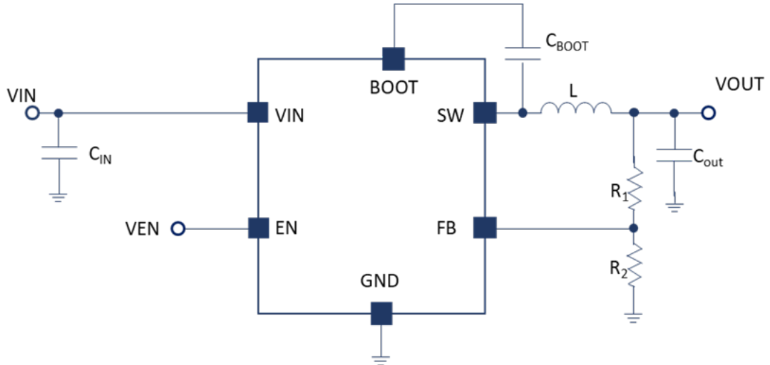
Figure 1. DCP3603 typical application schematic
