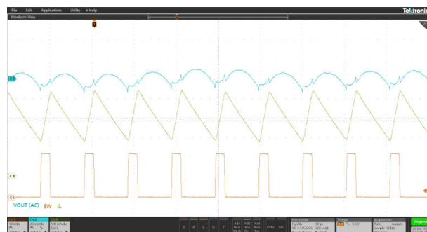
Figure 12. DCP3603BC - LCM operation at no load V_{IN} = 24 V, V_{OUT} = 5 V, I_{OUT} = 1.5 A
