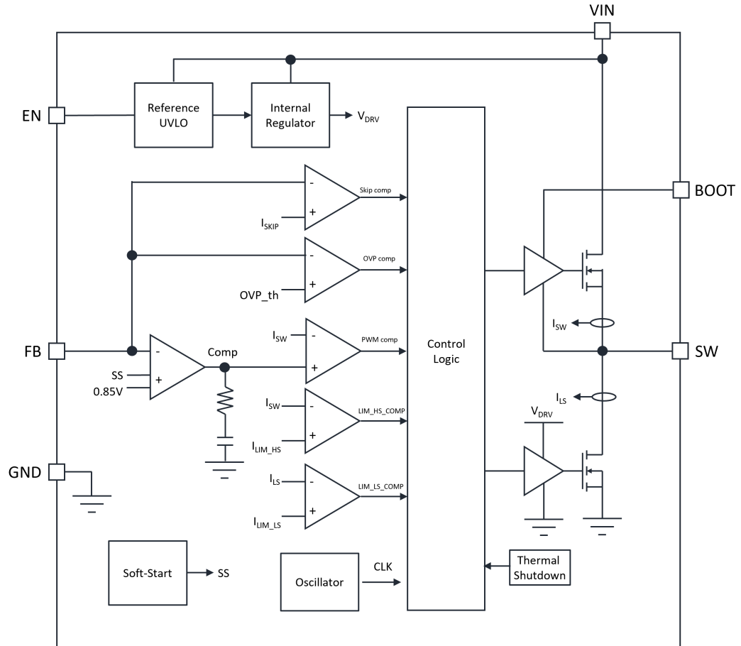
Figure 3. Simplified block diagram
