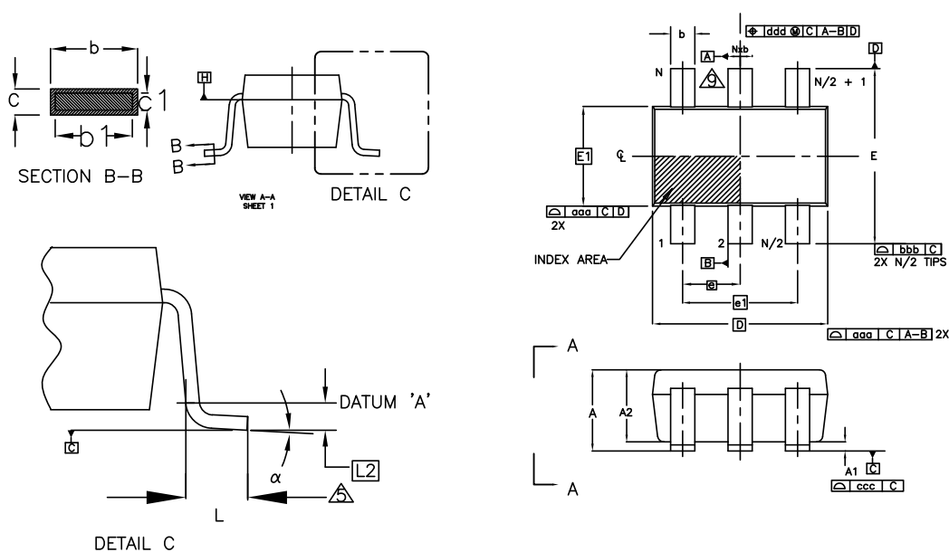
Figure 15. SOT23-6L package outline
