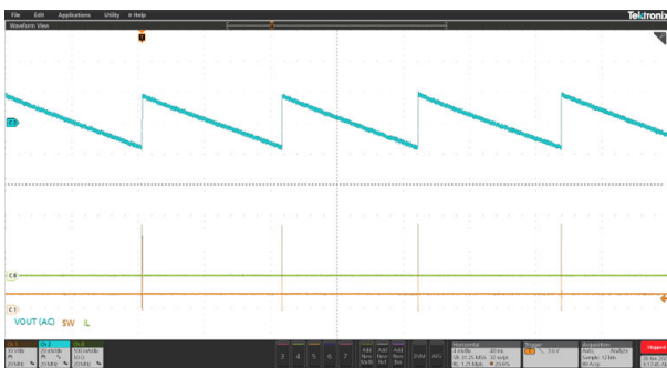
Figure 9. DCP3603AC - LCM operation at no load V_{IN} = 24\text{ V} , V_{OUT} = 5\text{ V} , NO LOAD
