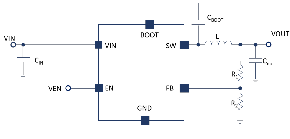
Figure 4. DCP3603 application schematic
