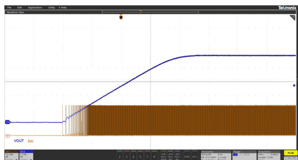
Figure 13. DCP3603AC SOFT-START phase V_{IN} = 24 V, V_{OUT} = 5 V, R_{LOAD} \approx 1.65 \Omega
