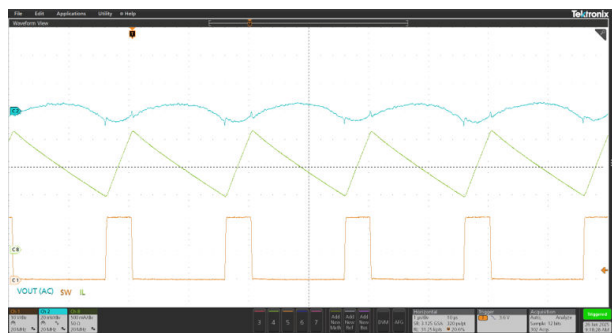
Figure 10. DCP3603AC - LCM operation at no load V_{IN} = 24\text{ V} , V_{OUT} = 5\text{ V} , I_{OUT} = 1.5\text{ A}
