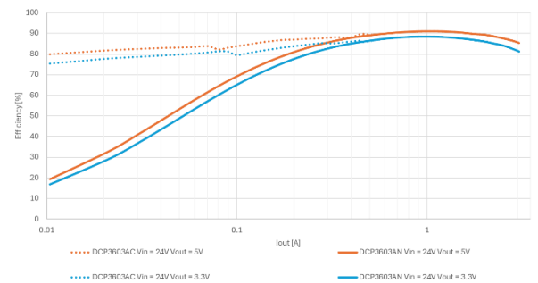
Figure 5. DCP3603A – Efficiency ( V_{IN} = 24\text{ V} )
