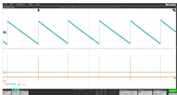
Figure 11. DCP3603BC - LCM operation at no load V_{IN} = 24 V, V_{OUT} = 5 V, NO LOAD
