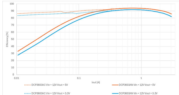
Figure 6. DCP3603A - Efficiency ( V_{IN} = 12\text{ V} )
