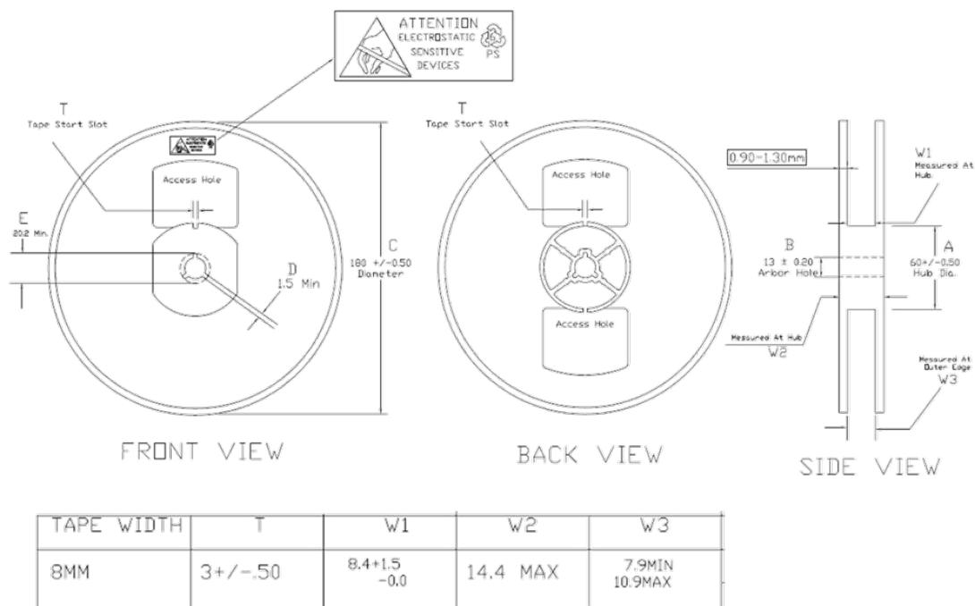
Figure 18. SOT23-6L reel outline
