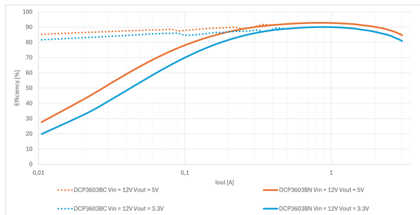
Figure 8. DCP3603B – Efficiency ( V_{IN} = 12\text{ V} )
