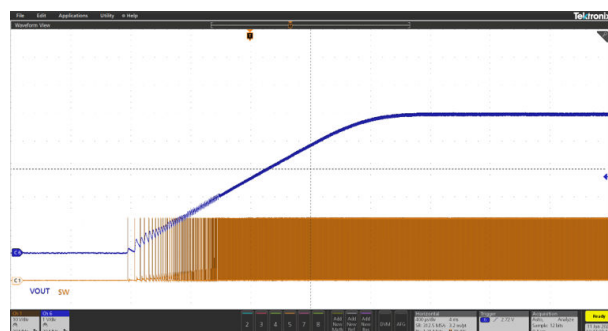
Figure 14. DCP3603BC SOFT-START phase V_{IN} = 24 V, V_{OUT} = 5 V, R_{LOAD} \approx 1.65 \Omega
