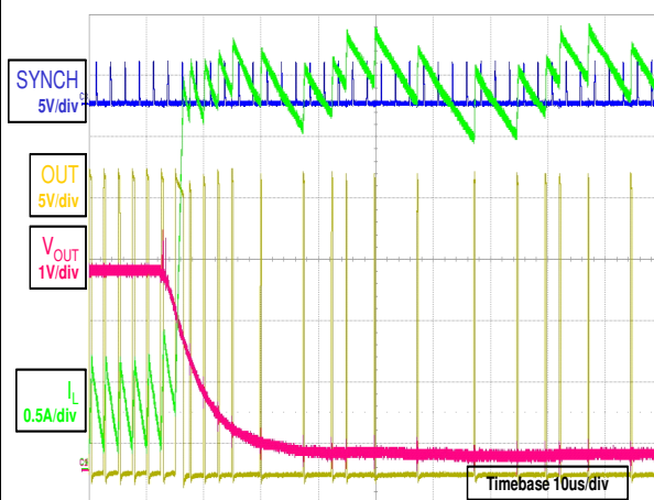
Figure 33. Short-circuit behavior at V_{IN} = 24V
