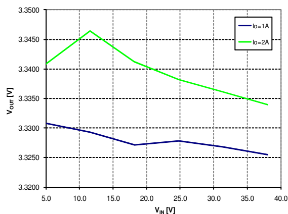
Figure 29. Line regulation
