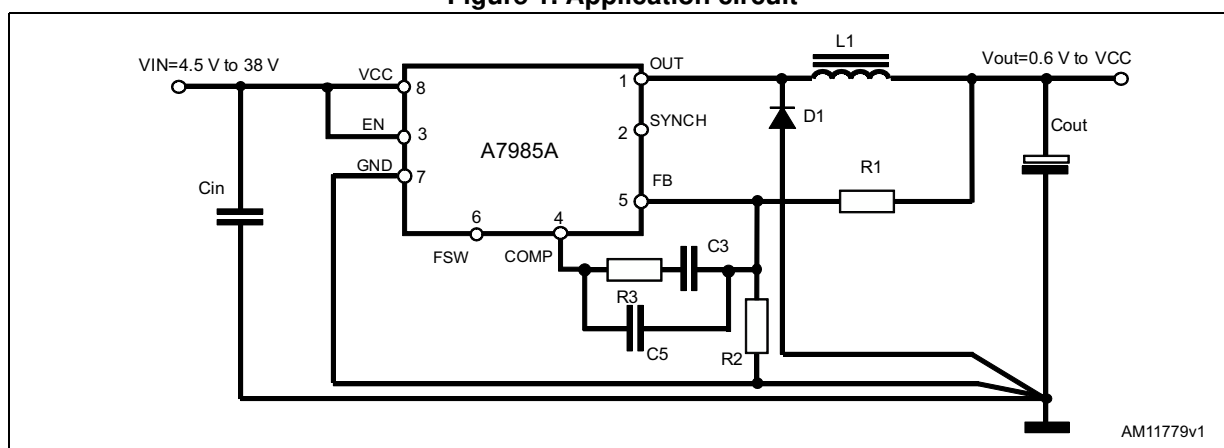
Figure 1. Application circuit
