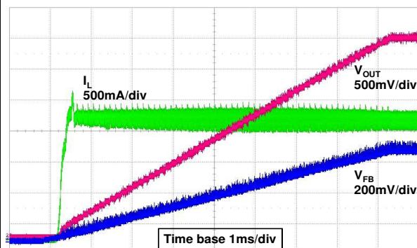
Figure 31. Soft-start
