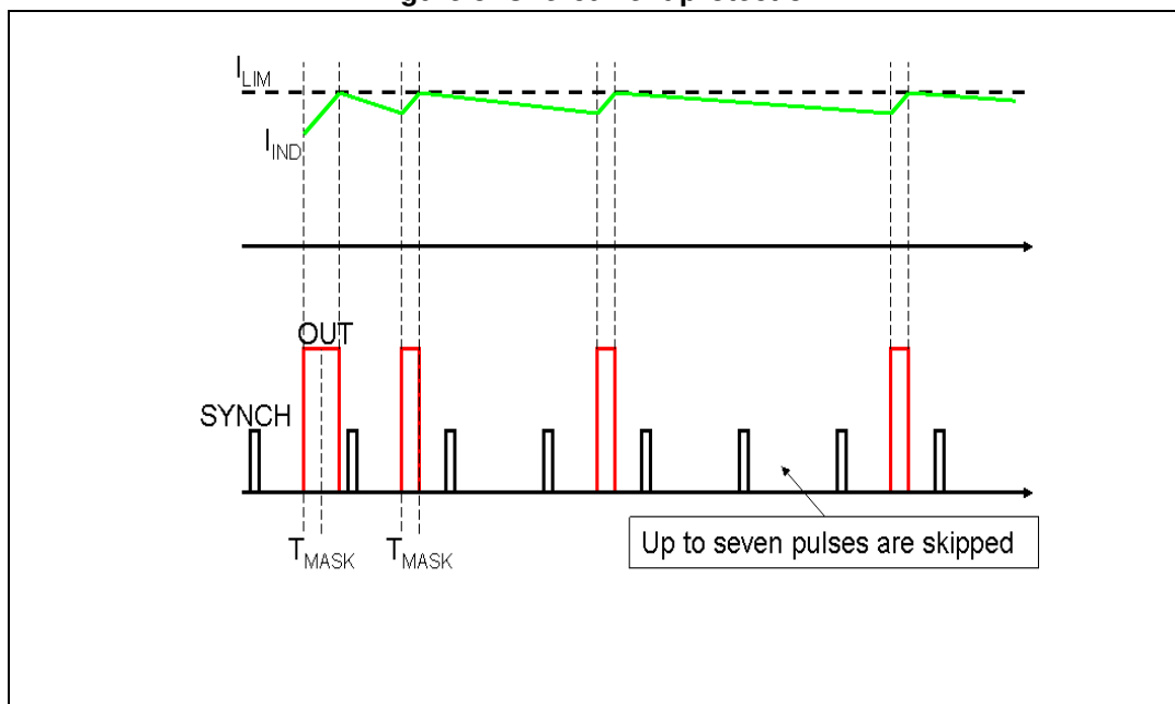
Figure 8. Overcurrent protection
