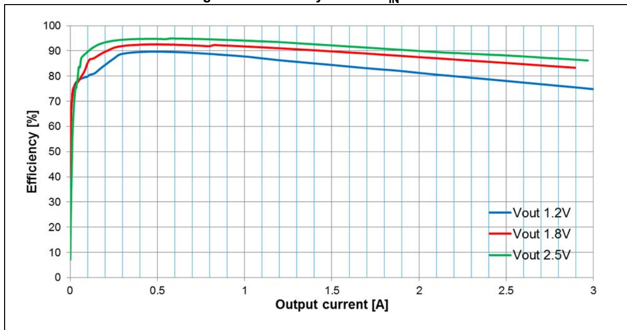
Figure 13. Efficiency curves: V_{IN} = 3.3\text{ V}
