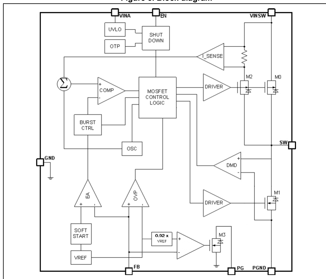
Figure 3. Block diagram
