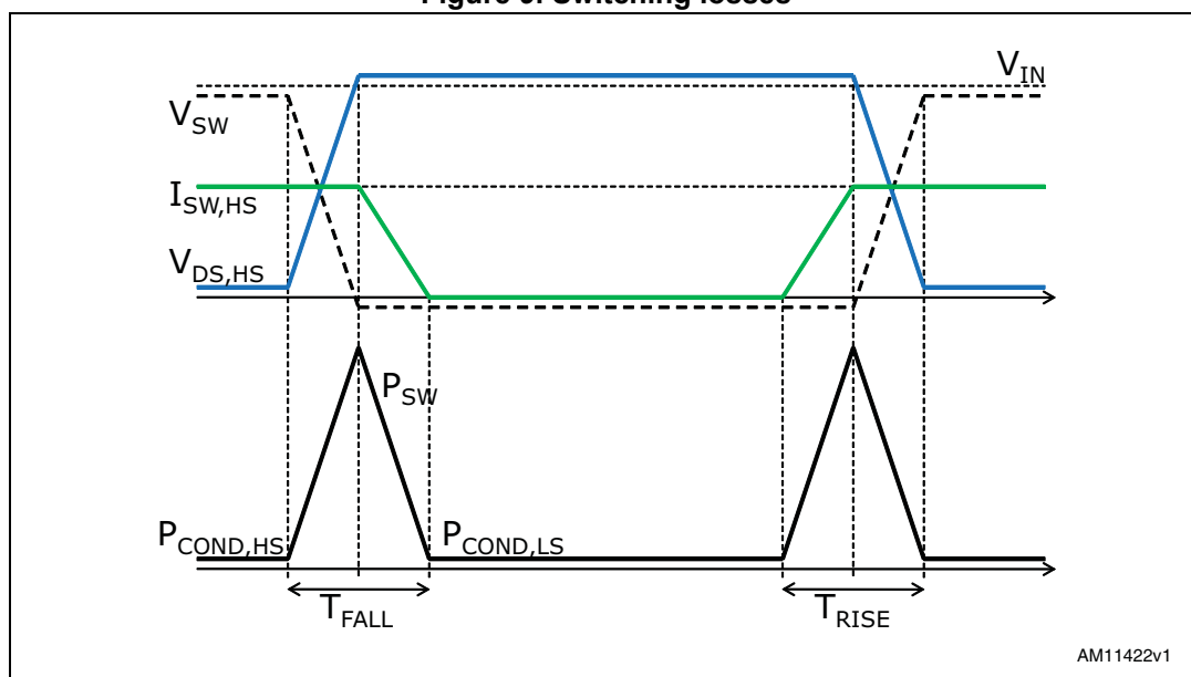
Figure 9. Switching losses
