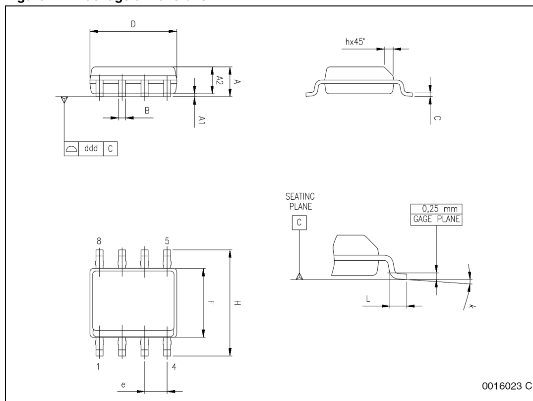
Figure 4. Package dimensions
