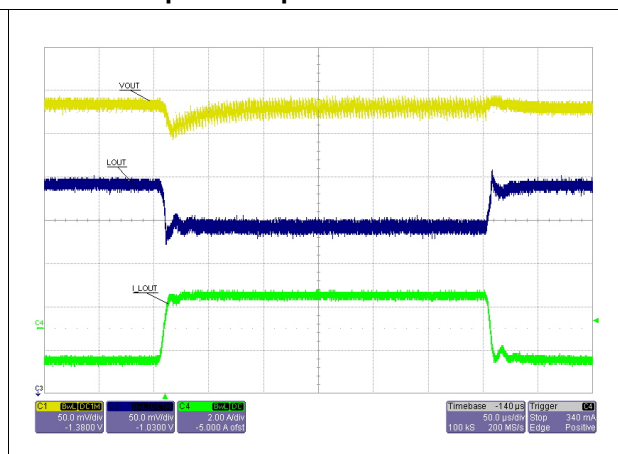
Figure 15. L_{OUT} load transient ( V_{IN} = 24V , LOAD = -1.5A \rightarrow 1.5A @2.5 A/μs). pulse-skip mode
