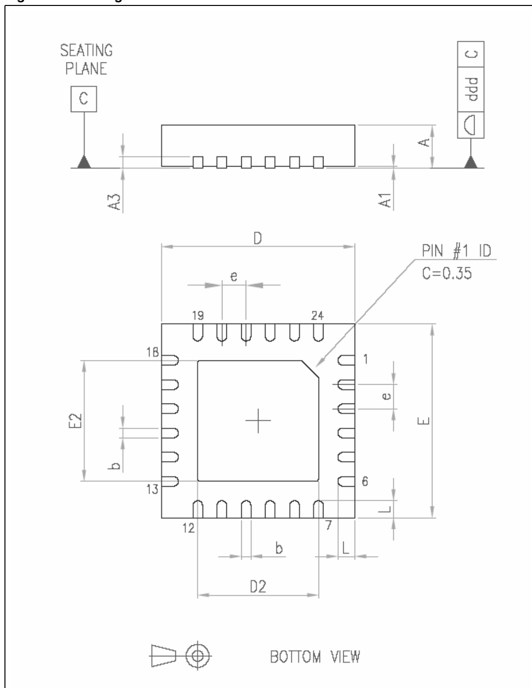
Figure 41. Package dimensions
