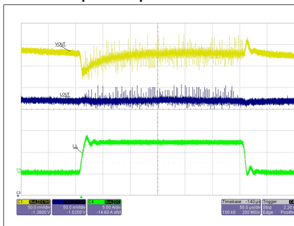
Figure 14. V_{OUT} Load Transient ( V_{IN} = 24V , LOAD = 0A \rightarrow 7A @2.5 A/μs). pulse-skip mode
