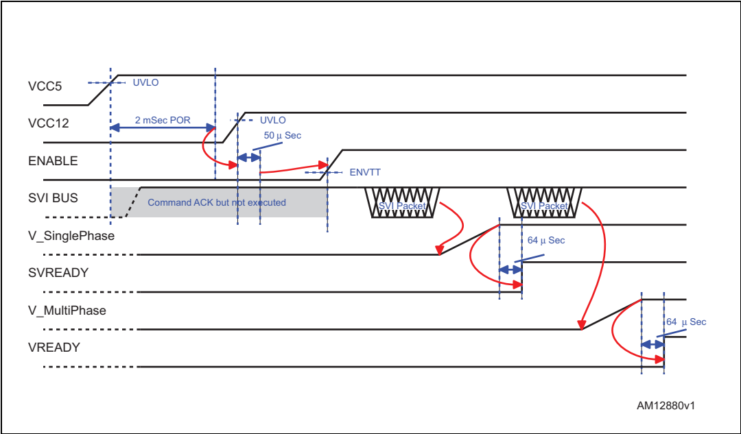
Figure 6. Device initialization
