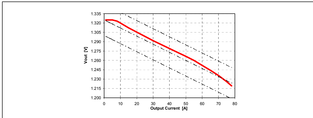
Figure 27. Load Regulation.
