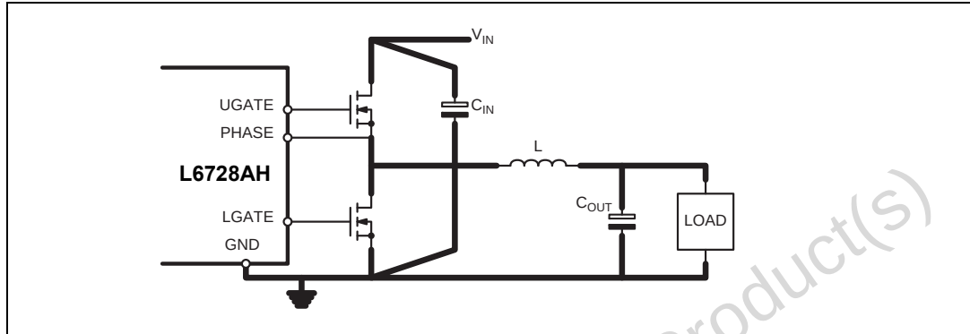
Figure 7. Power connections (heavy lines)
