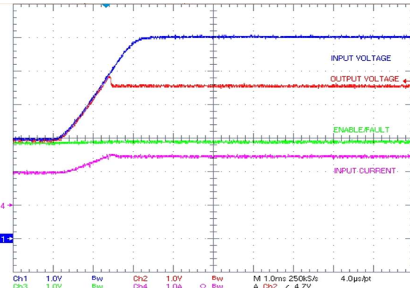
Figure 21. Voltage clamp
