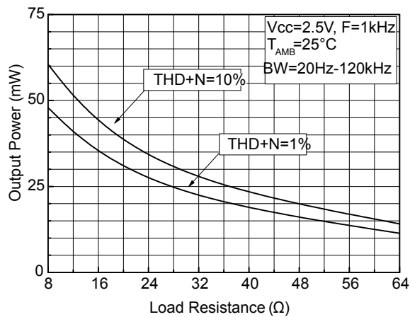
Figure 52. Output power vs. load resistance V_{CC}=2.5\ \text{V}
