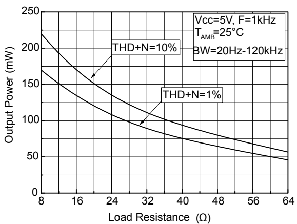
Figure 54. Output power vs. load resistance V_{CC}=5\ \text{V}
