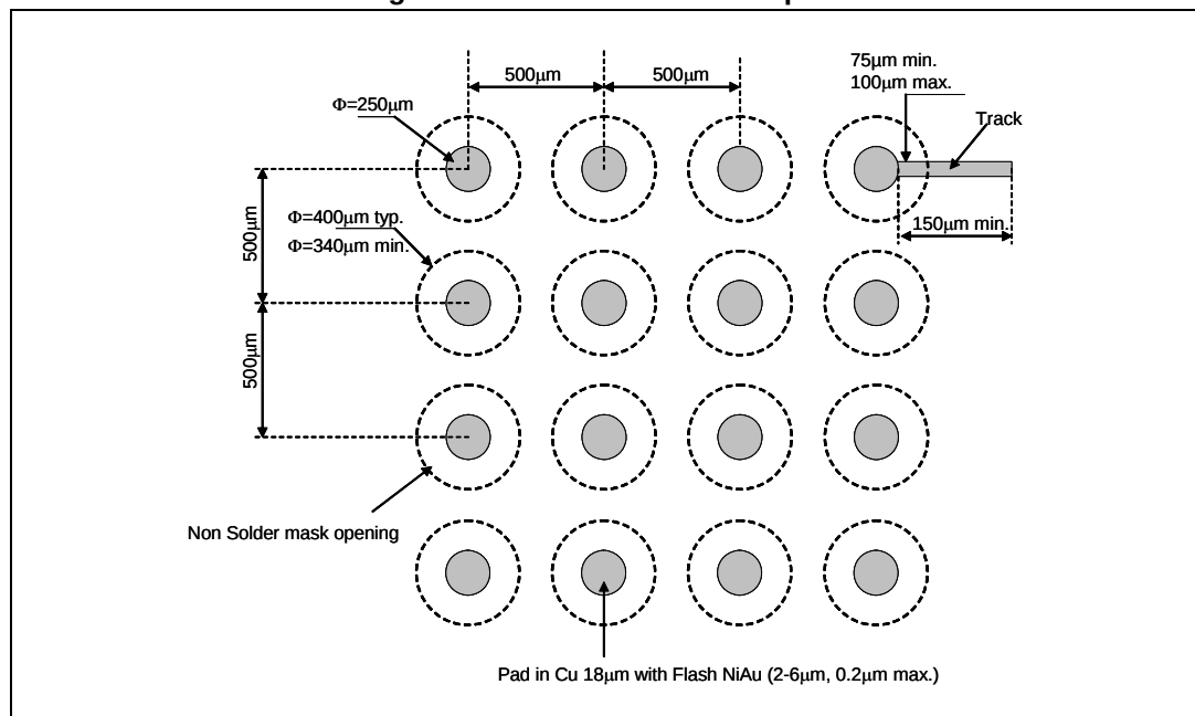
Figure 45. Recommended footprint
