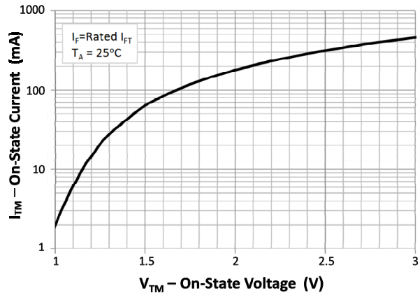
Fig 6 On-state Current On-state Voltage
