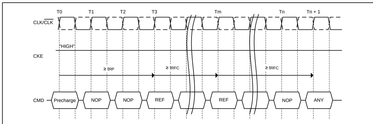
Figure 13 – Refresh command
