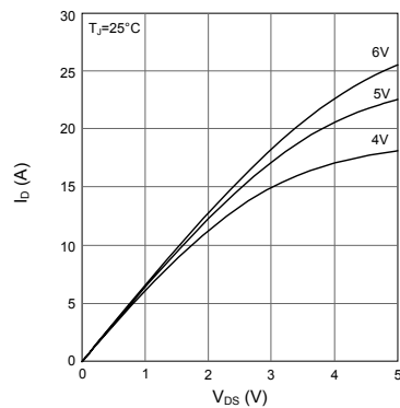
Figure 4. Typ I_D vs. V_{DS} at T_J = 25^\circ\text{C}
