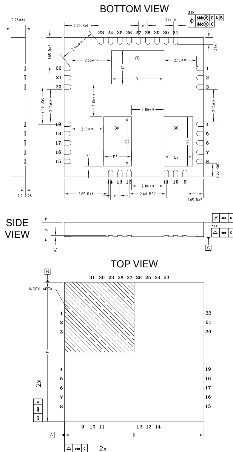
Figure 22. QFN 9 x 9 x 1 mm package dimensions
