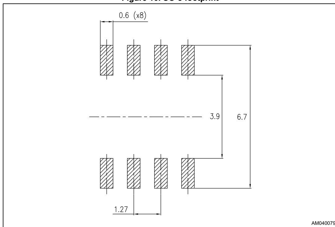
Figure 10. SO-8 footprint
