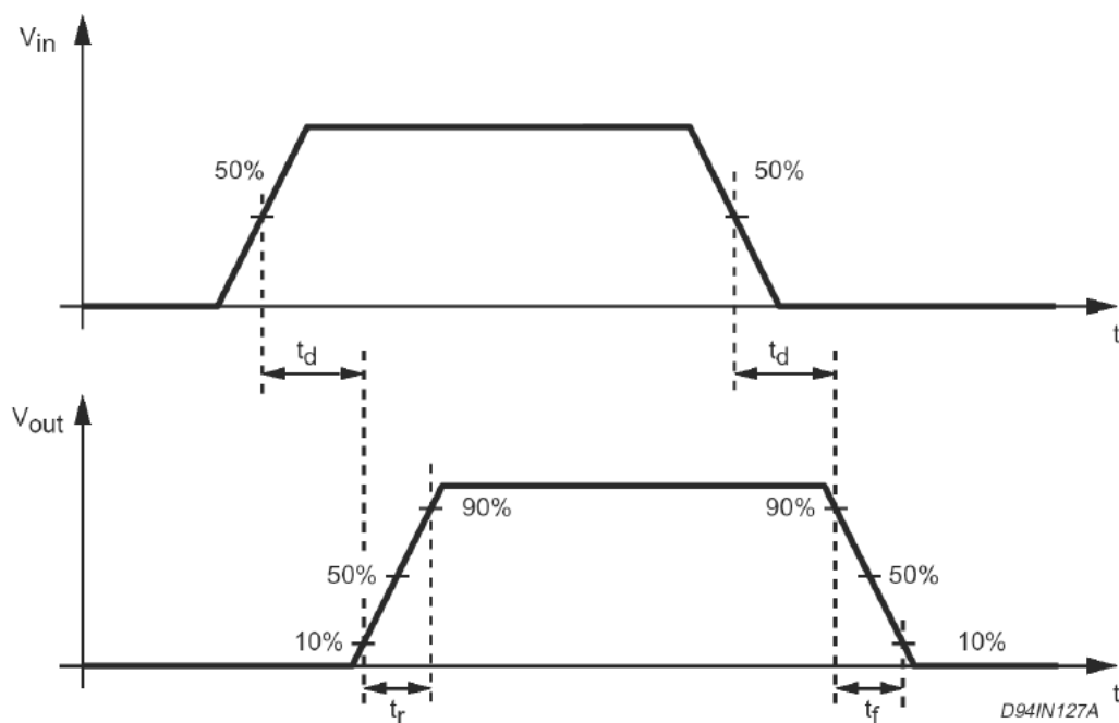
Figure 3. Switching waveforms
