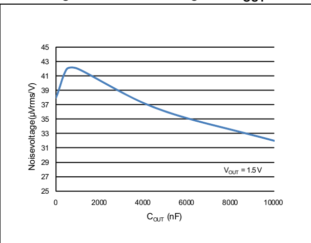
Figure 14. Noise voltage vs. C OUT
